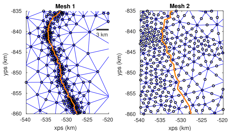
Figure B1. Exemplary zoom into the Bindschadler grounding line for two different meshes. Left panel: elements and nodes of the mesh presented in the main text. The mesh was refined especially around the grounding line and linear 3-node elements were employed. Right panel: alternative mesh with 6-node elements with quadratic base functions. The grounding line position is indicated in both meshes in orange.
