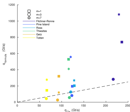
Figure B3. Comparison of fluxes calculated with Ua (x-axis) and with the analytical flux formula (y-axis), integrated along the grounding lines of exemplary ice shelves. Symbols indicate the different sliding law exponents m = 1, 3, 7 employed. All other parameters agree with the reference run (indicated by a circle). The dotted line shows where fluxes calculated with Ua and predicted by the formula would agree.
