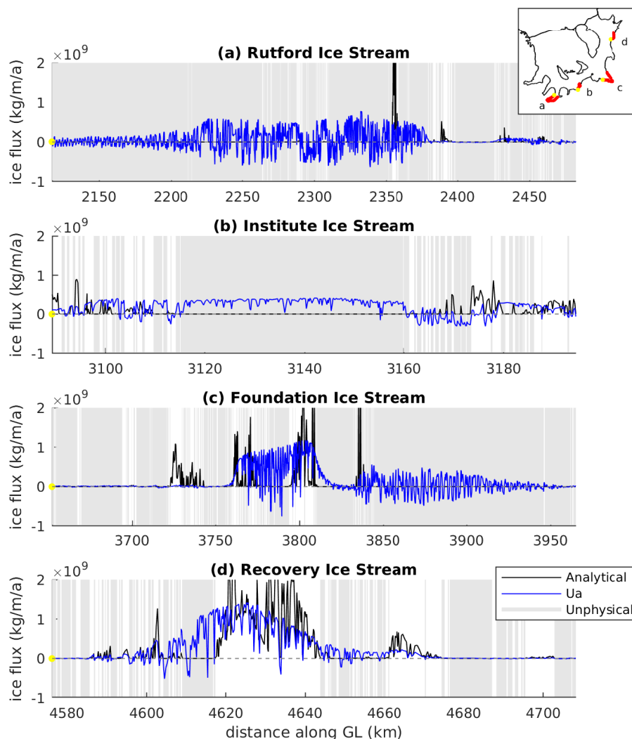
Figure 4. Comparison of fluxes calculated with \hat{U}_a (blue) and analytical fluxes (black) along the grounding lines of four major ice streams draining into Filchner-Ronne Ice Shelf. Locations where the flux formula provides unphysical results are marked in grey. Plotted grounding line segments are located as displayed in the inset with western margins indicated by a yellow dot.
