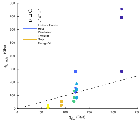
Figure B4. Comparison of fluxes calculated with \dot{U}_a (x-axis) and with the extended flux formula (y-axis), integrated along the grounding lines of exemplary ice shelves. Symbols indicate the different definitions of \theta as described in Sect. 2. All other parameters agree with the reference run (indicated by a circle). The dotted line shows where fluxes calculated with \dot{U}_a and predicted by the formula would agree.
