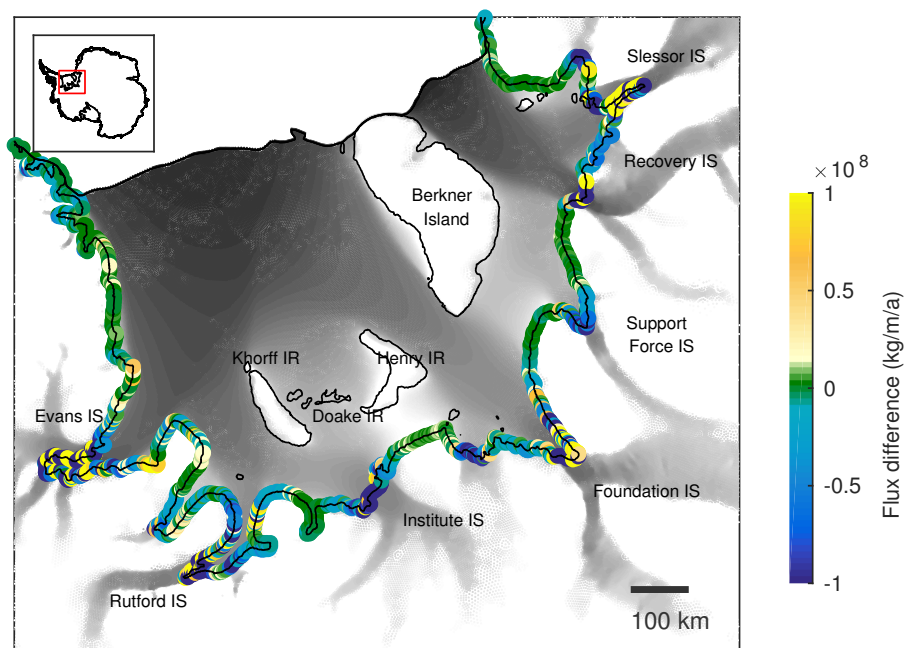
Figure B2. Difference between formula-derived and modeled fluxes along the grounding lines of Filchner-Ronne Ice Shelf. In contrast to Fig. 5 a different mesh was employed (exemplified in the right panel in Fig. B1), the data assimilation was conducted using Bayesian inversion and based on the MEASURES velocity data set (Rignot et al., 2011). The analysis was done using quadratic elements. This Antarctic-wide setup is described in more detail in Reese et al. (2017).
