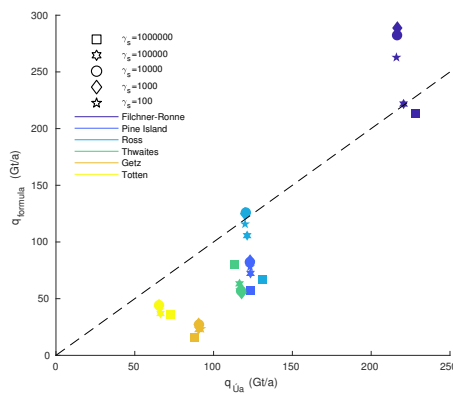
Figure B5. Comparison of fluxes calculated with \dot{U}_a (x-axis) and with the extended flux formula (y-axis), integrated along the grounding lines of exemplary ice shelves. Symbols indicate the different regularization parameters \gamma_s used. All other parameters agree with the reference run (indicated by a circle). The dotted line shows where fluxes calculated with \dot{U}_a and predicted by the formula would agree.
