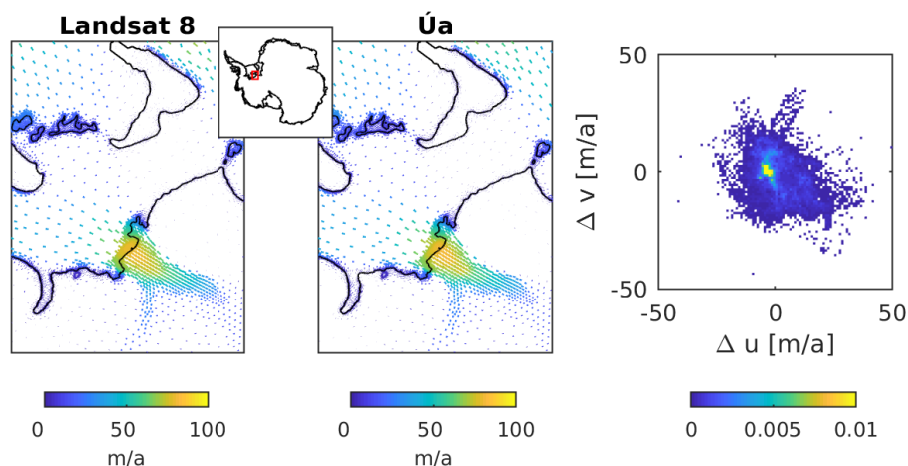
Figure 1. Observed (left panel) and modelled (middle panel) ice velocities in the region of Institute Ice Stream. The inset displays the location of the plotted area in Antarctica. Grounding lines are shown as black lines and colorscales indicate the speed. The right panel shows a normalised bivariate histogram of the velocity residuals which are the differences between modeled and observed velocities within this area, that is, \Delta u = u_{\text{modeled}} - u_{\text{observed}} and \Delta v = v_{\text{modeled}} - v_{\text{observed}} , and u and v are the horizontal components of the surface velocity vector, respectively.
