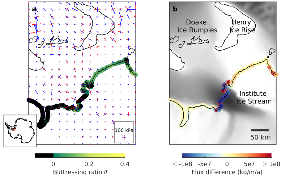
Figure 3. Butting ratio and differences in grounding line flux for Institute Ice Stream draining into the Filchner-Ronne Ice Shelf (location shown in inset). (a) Butting values \theta_1 are displayed along the grounding line and principle deviatoric stresses are shown, with compression in red and extension in blue. The length of the vectors indicate the magnitude of each principle stress. (b) Differences between analytical and modeled fluxes and observed ice velocities ranging up to 500 \text{ m a}^{-1} (Gardner et al., 2017). Analytical fluxes are set to 0 where \theta_1 < 0 . Grounding line positions are indicated in black.
