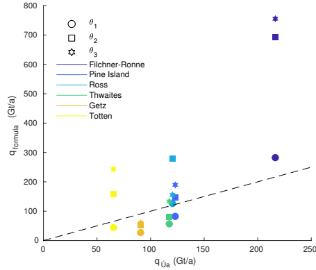
Figure B4. Comparison of fluxes calculated with \dot{U}a ( x -axis) and with the analytical flux formula ( y -axis), integrated along the grounding lines of the ice shelves indicated in the legend. Symbols indicate the different definitions of \theta as described in Sect. 3. All other parameters agree with the reference run (indicated by a circle). The dashed line shows where fluxes calculated with \dot{U}a and predicted by the formula would agree.
