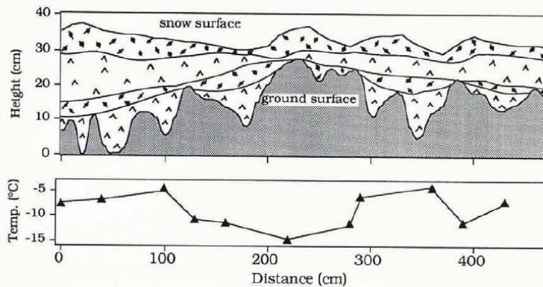
Fig. 2. A cross section through the snow cover at Innavait Creek, 18 November 1989. Depth hoar is indicated by an inverted “V”; wind slab is indicated by a dot with a line through it. Note discontinuous snow strata that pinch out over tussock tops. In the lower part of the figure, the temperature of the snow/ground interface is shown.
