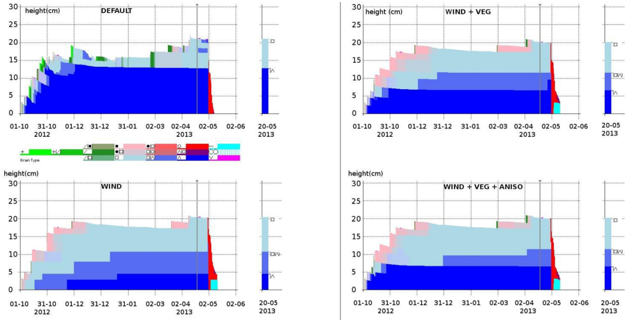
Figure 6: SNOWPACK grain shapes in the 4 simulation setups. The colour code was complemented with grain shape symbols after Fierz et al. (2009) for the 20-05-2013 profile (as representative of the time of the snow campaign).
