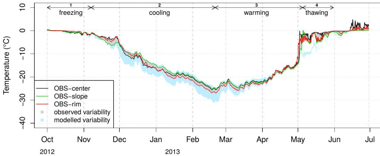
5 Figure 10: Simulated and observed soil temperature variability (in °C) at 5 cm depth. Observed soil temperatures at rim, center and slope locations in the reference polygon are overlain.
