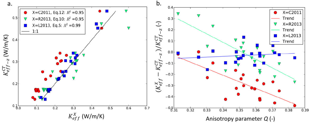
Figure 5 : a. Comparison between estimates of K_{eff} or K_{eff-z} made with the CT method ( K_{eff-z}^{CT} ), and estimates made using parameterization "X" ( K_{eff}^X , where X=C2011, R2013 or L2013: see manuscript for description of these parameterizations). b. Relative bias in K_{eff}^X with respect to K_{eff-z}^{CT} as a function of the anisotropy parameter Q. Each point represents a snow sample analysed by CT in this study.
