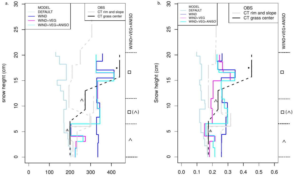
5 Figure 7: Observed and simulated density and K_{eff-z} profiles on 20-04-2013. Observations (OBS) are the estimates made using the CT method at the three CT sites with basal vegetation; grain shape is indicated on the plot for the CT grass-center site. Simulations (MODEL) were made with the four SNOWPACK setups; grain shape is indicated at the side for the WIND+VEG+ANISO setup.
