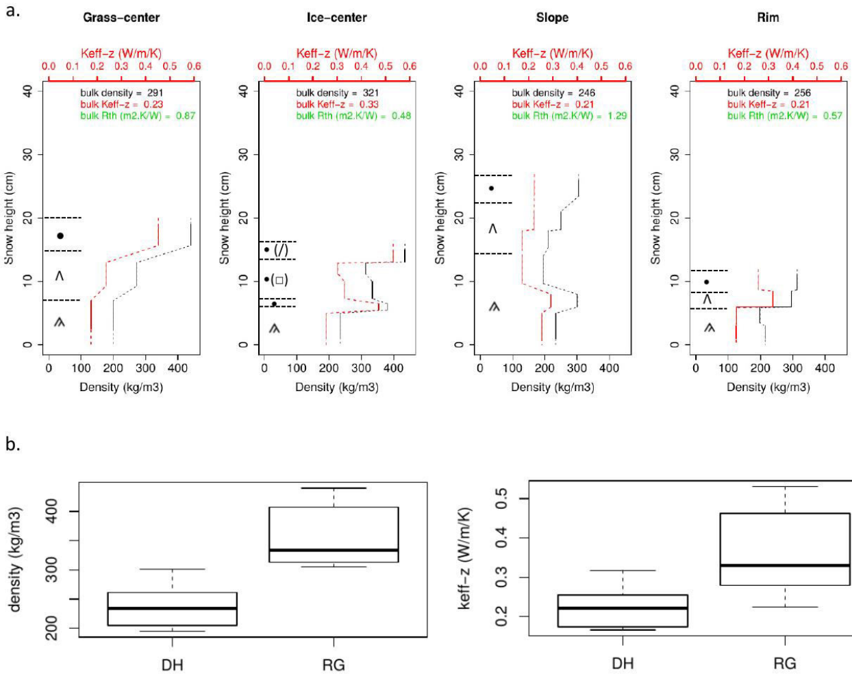
Figure 3: (a) Grain shape, density and K_{eff-z} profiles from the four CT sites. Density and K_{eff-z} values are represented by piecewise constant functions over the layers where the CT analysis was performed; these segments are connected by a dashed line as a guide to the eye. Symbols for the grain shapes originate from Fierz et al. (2009). When several grain shapes coexist within a layer, the dominant type is listed first. (b) Boxplots of density and K_{eff-z} for individual DH layers (11) and rounded grain (RG) layers (8) found within the CT profiles. RG shapes were occasionally associated with faceted crystals and decomposing and fragmented precipitation particles.
