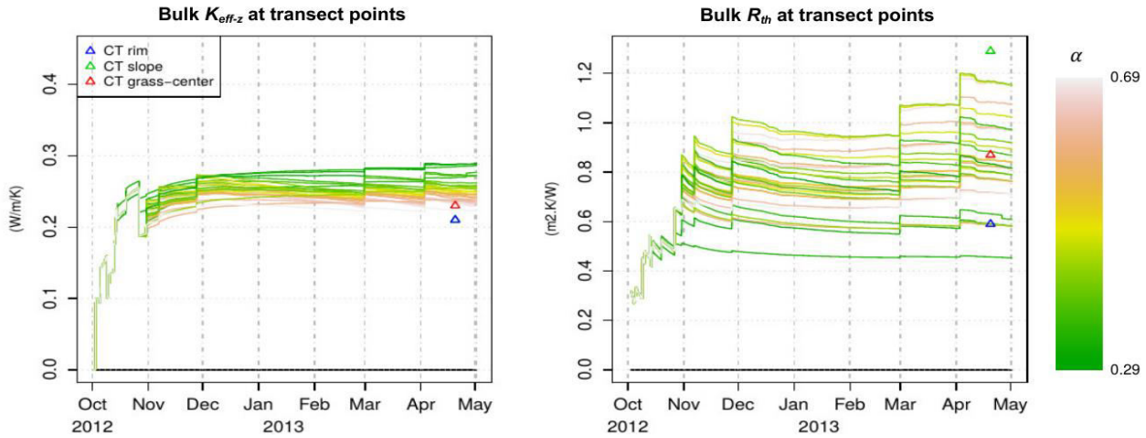
Figure B2: Simulated K_{eff-z} and R_{th} time-series at the 31 transect data points. Overlain are the bulk properties estimated at the rim, slope and grass-center CT sites.
