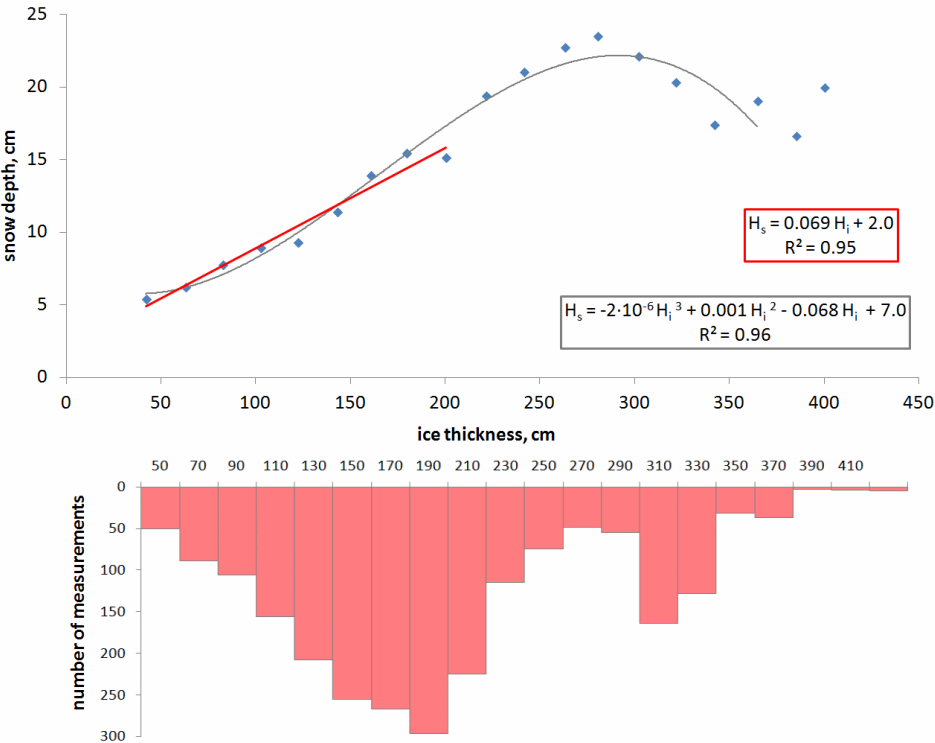
Figure 7. The relation between the thickness of the undeformed ice and the depth of accumulated snow in the end of winter. The next step in the analysis of the Sever data was focused on the local variations of snow depth caused by wind action and ice deformation, leading to formation of sastrugi, hummocks and snow dunes. As described in Sect. 2, measurements of snow depth of sastrugi (sastrugi height), snow depth on hummocks and depth of snow dunes connected to ice ridges have been done at a significant number of landings (Fig. 3). That data allows us to evaluate local variations of snow depth on single floes and to analyze spatial variability of snow irregularities over larger areas.
