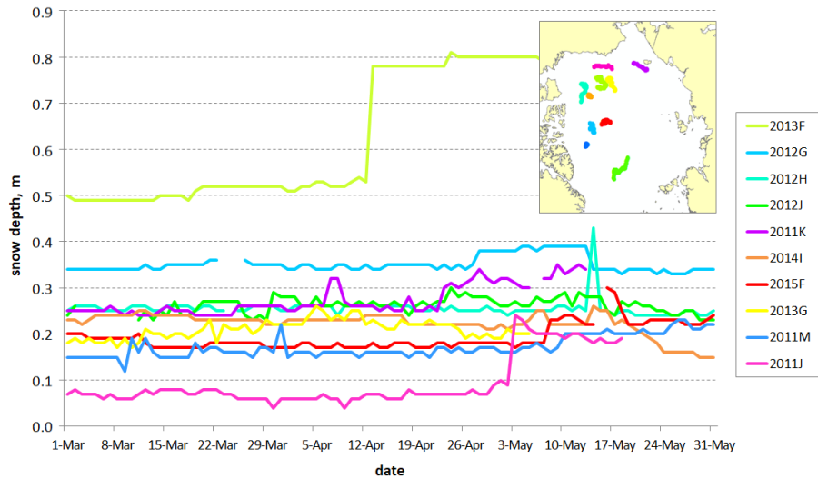
Figure 12. IMB observations of snow depth in the MAM months, 2012-2016, provided by CRREL. The number before a letter in the buoy's name indicates the year when the buoy has been deployed. Tracks of the buoys in the MAM months are shown on the map.
