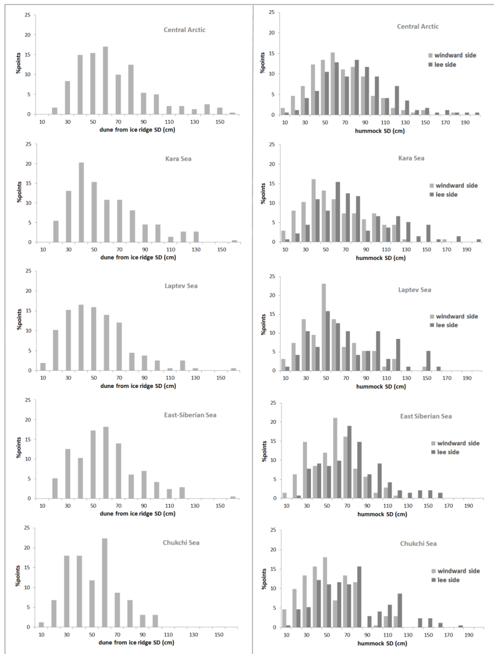
Figure 9. Distribution functions of snow depth (SD) in the dunes attached to ice ridges and around hummocks (on the windward and on the lee side) in different parts of the Arctic.
