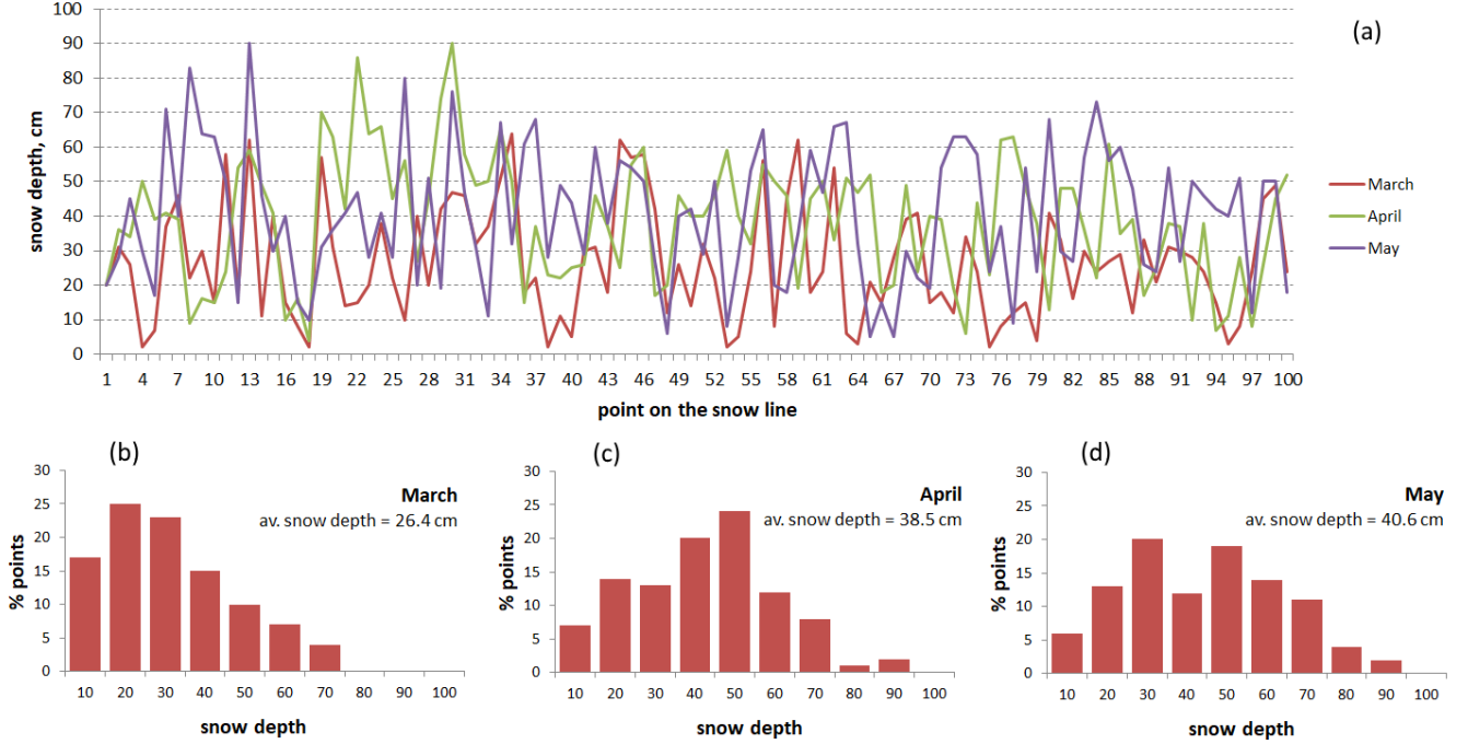
Figure 10. (a) Snow line measurements made in 1969 in the MAM months during the work of NP16 drifting station. The length of snow line was 1 km. (b) - (d) Distributions of measured snow depths in March, April and May 1969.
