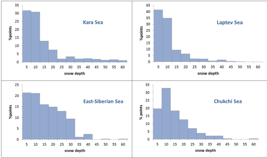
Figure 6. Distribution of snow depth on the level ice in the marginal seas. The snow depth in the Kara and Laptev seas is dominated by snow depth up to 10 cm, indicating prevalence of FY ice. The Kara Sea also has cases of very thick snow cover, which can be explained by high density of data in the north-eastern part of the Kara Sea as shown in Fig 5. Snow conditions observed in that area were highly variable, which is explained by very condensed observations that captured a wide variety of ice and snow characteristics in that region. On average, the East-Siberian and Chukchi seas had more observations of thicker snow cover, which agrees with the higher proportion of MY ice in these regions. The start time of snow accumulation is one of the major factors determining the snow depth by the end of snow accumulation season (Radionov et al., 1997; Hezel et al., 2012). In the case of FY ice, snow accumulation can only start after the sea ice freezing is stable. A delayed sea ice freeze-up will lead to a delayed start of snow accumulation and thereby have impact on the snow depth evolution during the winter (Webster et al., 2014). MY ice begins to accumulate snow earlier in the fall; additionally, in some regions the snow can survive through the summer season. The ice thickness generally increases throughout the cold season, and though the sea ice growth rate is known to be inversely proportional to its thickness (e.g., L’Heveder and Houssais 2001, Bitz and Roe, 2004) we would expect the ice thickness to be related to the depth of snow
