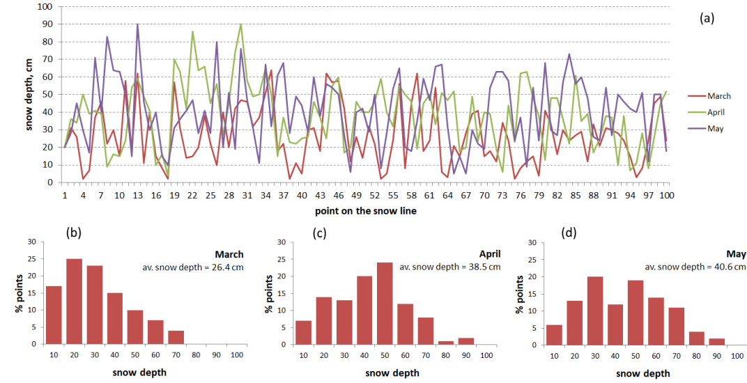
Figure 10. (a) Snow line measurements made in 1969 in the MAM months during the work of NP16 drifting station. The length of snow line was 1 km. (b) - (d) Distributions of measured snow depths in March, April and May 1969.
