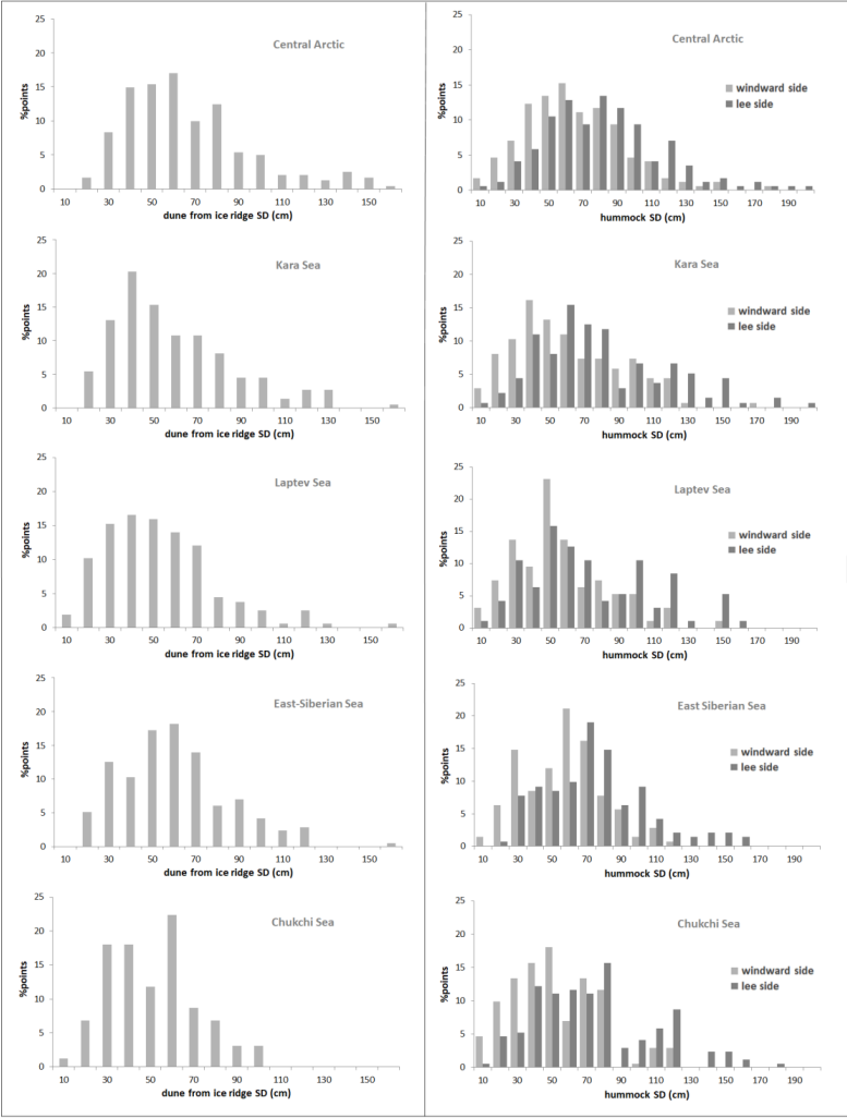
5 | Figure 9. Distribution functions of snow depth (SD) in the dunes attached to ice ridges and around hummocks (on the windward and on the lee side) in different parts of the Arctic.
