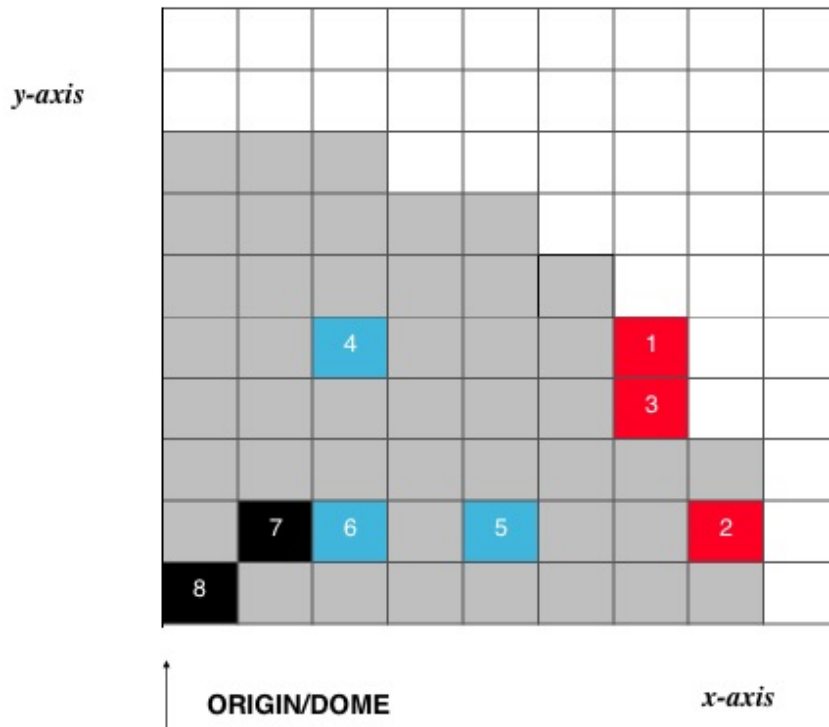
Figure 5. Grid map used to interpret the following box-plots in Figure 6. Eight randomly chosen grid points are selected for testing predictions; these are not the same as the measurement locations. Only one quadrant of the glacier is shown due to symmetry as is done in Figures 9,10, and 12 of Bueler et al. (2005), and the width of each cell is 10^5 m. Additionally, the red squares indicate locations at or close to the margin, the blue squares indicate locations that are between the dome and margin of the glacier, and the black squares indicate locations at or close to the dome of the glacier. Moreover, glacier grid squares with non-zero thickness are shaded in grey, as to indicate the glacier location.
