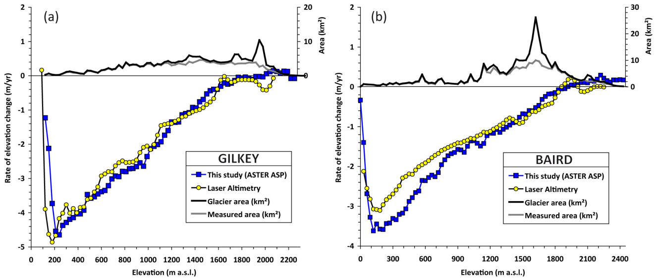
Supplementary Figure S1: Rates of elevation change vs. elevation for (a) Gilkey Glacier (Juneau Icefield) and (b) Baird Glacier (Stikine Icefield) measured from ASTER DEMs (blue curve, 2000-2016) and airborne laser altimetry data (2007-2012 for Gilkey and 1996-2013 for Stikine). The upper curve (right Y-axis) show the total area altitude distribution (black) and the glacier area effectively sampled using in the ASTER dh/dt (grey).
