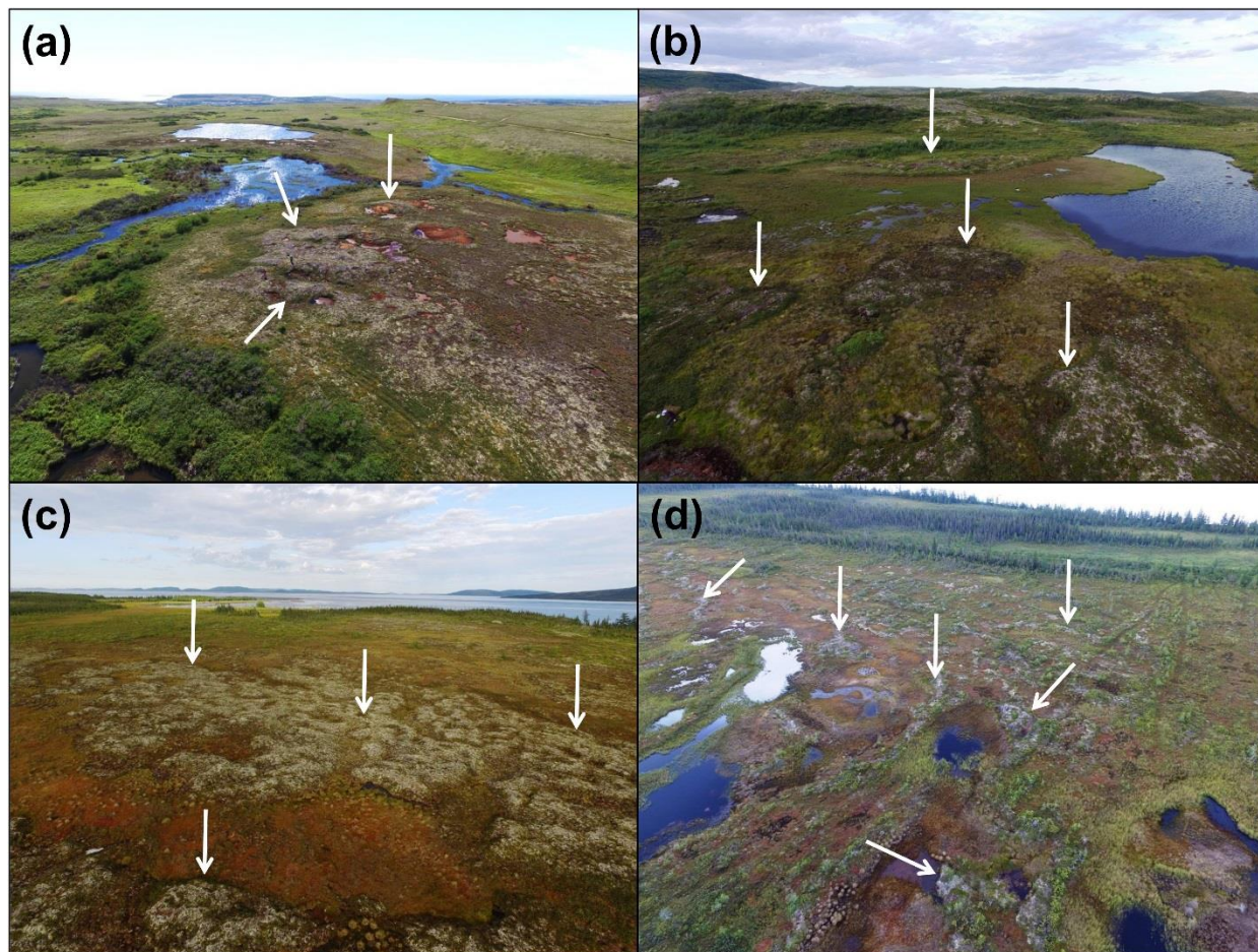
Figure 2. Low altitude UAV imagery of peatland permafrost sites at (a) Blanc Sablon, QC; (b) Red Bay, NL; (c) Main 5 Tickle, NL; and (d) Neveisik Island, NL. White arrows point to examples of permafrost-cored mounds.
