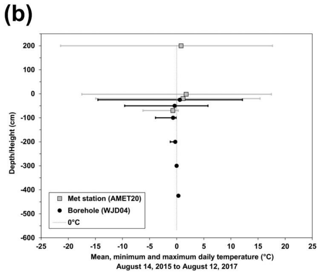
5 Figure 4. Peatland permafrost at Red Bay. (a) Frost tables and modelled resistivities on ERT profile 3. Depths with permafrost in borehole WJD04 are denoted by hatching; (b) Air and ground temperature envelopes (2015-2017); (c) UAV vertical image of the site. Black line delimits the approximate location of the ERT survey line and text shows the start and end points.
