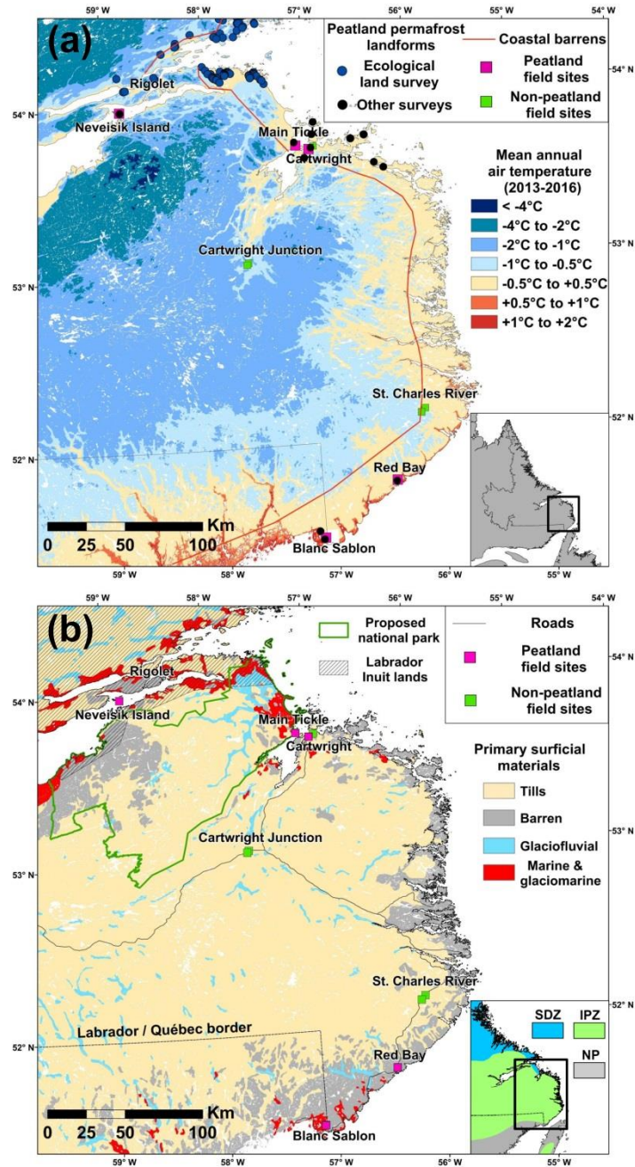
5 Figure 1. Location of peatland and non-peatland study sites in southeastern Labrador in relation to: (a) gridded (100 m resolution) mean annual air temperatures (2013-2016) (Way et al., 2017) and peatland landforms mapped in various studies, and (b) surficial materials (Fulton, 1995). The inset map in (a) shows the study location in eastern Canada and the boundary of the coastal barrens ecozone (Roberts et al., 2006) is shown as an orange line. Labrador Inuit lands and the proposed Mealy
