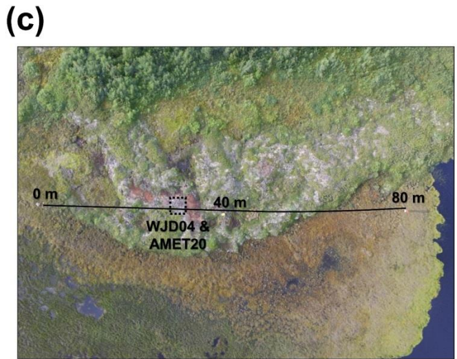
5 Figure 4. Peatland permafrost at Red Bay. (a) Frost tables and modelled resistivities on ERT profile 3. Depths with permafrost in borehole WJD04 are denoted by hatching; (b) Air and ground temperature envelopes (2015-2017); (c) UAV vertical image of the site. Black line delimits the approximate location of the ERT survey line and text shows the start and end points.
