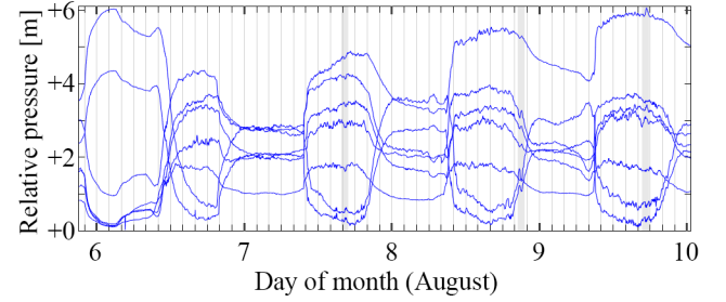
Figure 10. Relative pressure variations in 7 boreholes (orange symbols in Fig. 2) displaying common small amplitude diurnal oscillations with high-frequency content during August 2011. To make these visible in the same plot, we have applied offsets of 93, 71, 64, 61, 63, 66 and 27 metres to the measured pressures. Three common high-frequency features are highlighted by grey vertical bands.
