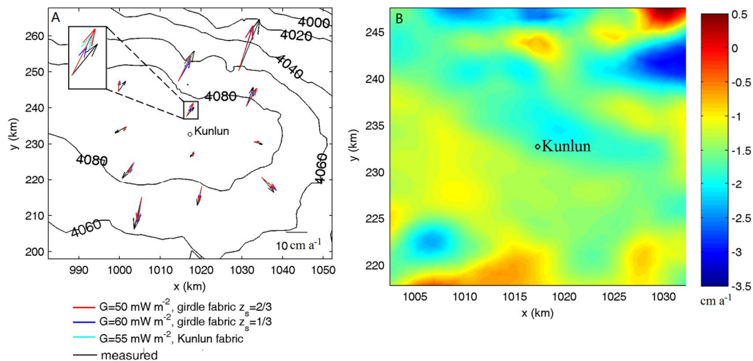
Fig. 7 (A) Surface topography with contours, and the measured (black arrows; Yang et al., 2014) and modeled surface horizontal velocity (see legend for details) near the Kunlun Station. Kunlun station is marked by a black circle. The coordinate system is WGS 1984 plotted using Antarctic Polar Stereographic with standard parallel at 71° S and central meridian at 0°E. The inset box is a zoom-in on one velocity datum showing the differences between ice fabrics. (B) Modeled surface vertical velocities (unit: cm a -1 ) using Kunlun fabric and a geothermal heat flux of 55 mW m -2 and surface temperature of -58.5°C. Note the region plotted in panel (B) is the central 30×30 km 2 area while in (A) it is the larger 70×70 km 2 region.
