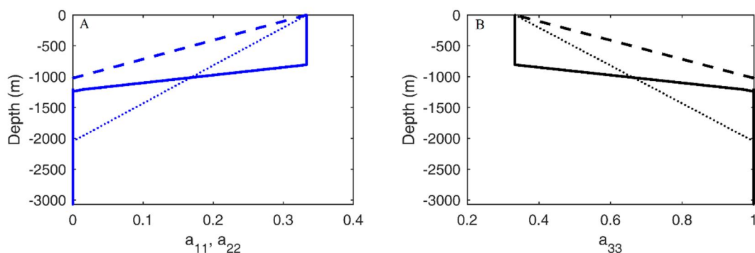
Fig. 2 Fabric as a function of depth (at Kunlun station) for Girdle fabric with z_s = 1/3 (dashed curve), and z_s = 2/3 (dotted curve), and Kunlun fabric (solid curve). The values of a_{11} (equals a_{22} ) are in blue in plot (A), while a_{33} is in black in plot (B).
