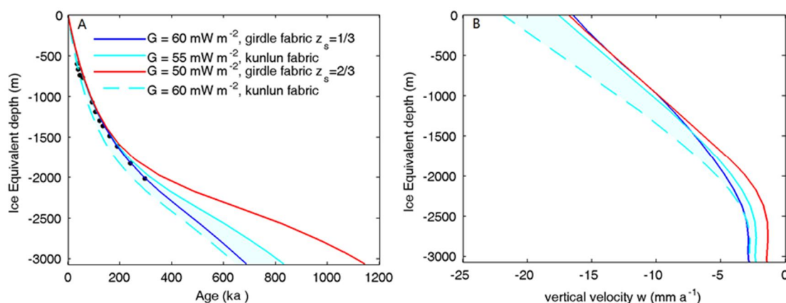
355 Fig. 3 The best-fit simulations (solid lines) at Kunlun station using geothermal heat fluxes of 50, 55 and 60 \text{ mW m}^{-2} . Modeled age–depth profile (A) and vertical velocity – depth profile (B). The black points denote the dated radar internal reflection horizons tracked from the Vostok ice core site, using a 37 m firm correction (based on the EDML ice core density profile, Ruth et al., 2007) subtracted from the radar depths to convert to the ice-equivalent model scale. The shaded cyan band shows an envelope of acceptable fits to the radar isochrones and age profile with depth, but the dashed ( 60 \text{ mW m}^{-2} ) line likely has too high surface velocities.
