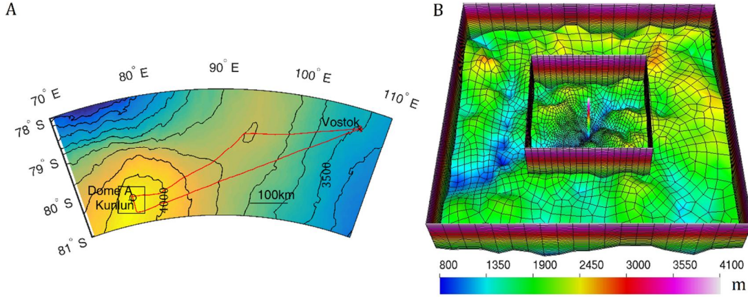
Fig. 1 (A) The locations of Dome A (black circle), Kunlun (black +), Vostok (black \times ) and the 70 \times 70 \text{ km}^2 study region (black box). The background is surface elevation with 100 m contour interval. The two radar lines that connect the Vostok drill site to Dome A are shown in red. (B) The 70 \times 70 \text{ km}^2 finite element mesh in the vicinity of Dome A projected on a polar stereographic map with standard parallel at 71^\circ \text{S} and central meridian at 0^\circ \text{E} . The background is bedrock elevation. The boundaries of the inner region and the whole region are shown, with the inner 30 \times 30 \text{ km}^2 region centred on Kunlun station has 300 m resolution, and the outer region 3 km resolutions. There are 21 terrain-following vertical layers with thinner layers near the base. The bar in the center denotes the drilling site at Kunlun station.
