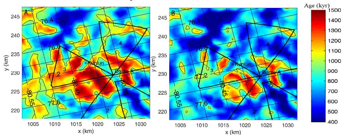
Fig. 6. Modeled age at the height of 200 m above the bedrock using Kunlun fabric and a geothermal heat flux of 55 (A) and 60 (B) \text{mW m}^{-2} in the standard grid coordinate system (unit: km, see Fig. 1), and WGS 1984 latitude and longitudes (inclined grid with the South Pole to the lower left). Kunlun station is marked by a black plus sign. The black curve is the 1 Ma age contour. The thick black line marks the polarimetric radar survey route triangles marked in Fig. 4.
