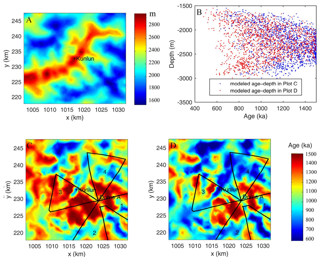
Fig. 5. 95 % depth in the central 30 \times 30 \text{ km}^2 model domain (A) and modeled age of the ice at this depth using Kunlun fabric and a geothermal heat flux of 55 (C, blue dots in plot B) and 60 (D, red dots in plot B) \text{mW m}^{-2} and surface temperature of -58.5^\circ\text{C} . The areas with no basal melt are arbitrarily limited to an age of 1.5 Ma. The black cross is Kunlun station. The black line marks the polarimetric radar survey route triangles marked in Fig. 4.
