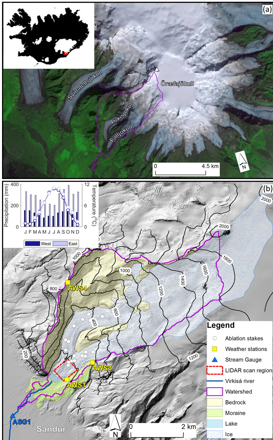
Figure 1. Location of Virkisá river basin on Örefajökull (top) and detailed topographical map of basin including major land surface types and observation data with inset showing mean monthly climate (bottom).
