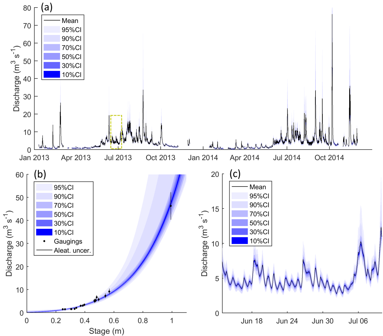
Figure 7. River flow time-series from ASGI with quantified confidence intervals (a), rating curve uncertainty used to quantify confidence intervals (b) and zoomed section of river flow time-series (see yellow dash box in top plot) with confidence intervals (c).
