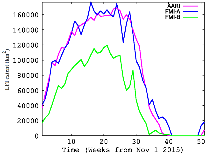
Figure 9. A LFI-area-times-Ice extent time series of AARI ice charts, FMI-A and FMI-B during the whole-study-one-year period from October 15-November 1 2015 to August 30 2017 until October 31, using the 2016. The time series is weekly with FMI-A and FMI-B algorithm for the same days as the weekly AARI ice charts.
