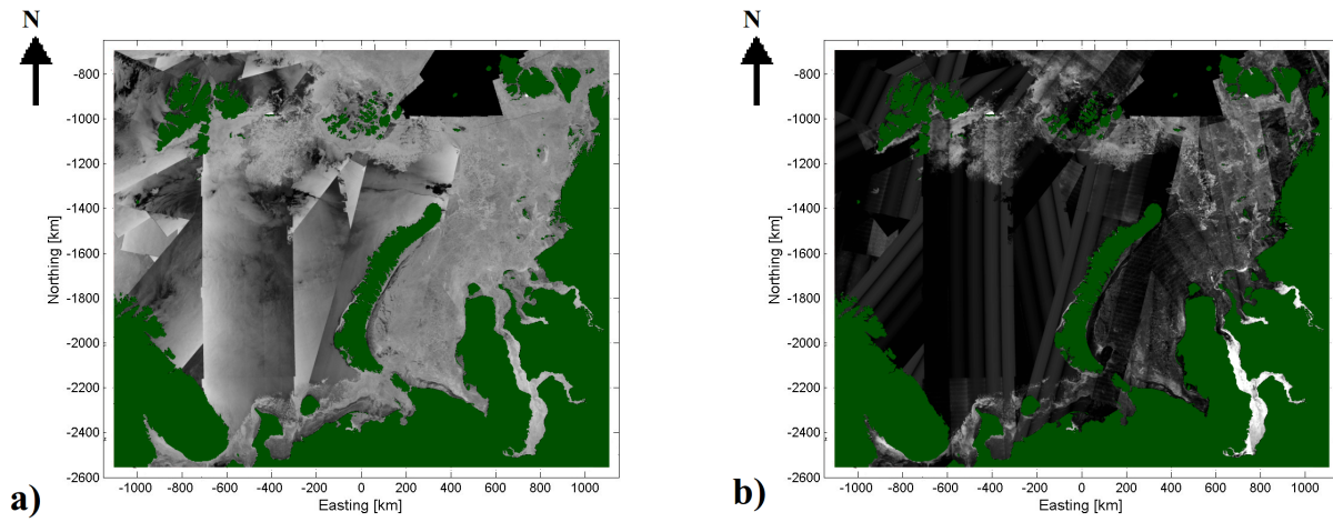
Figure 2. SAR mosaics of March 8, 2016, HH mosaic (left panel a) and HV mosaic (right panel b). The land areas, based on our land mask, appear as green and areas of no data are as black in the mosaics figures.
