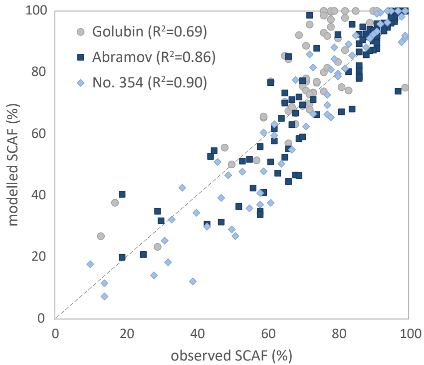
Fig. 2. Comparison between the observed SCAF and the modelled SCAF for Abramov (squares), Golubin (circles), and Glacier No. 354 (diamonds).
