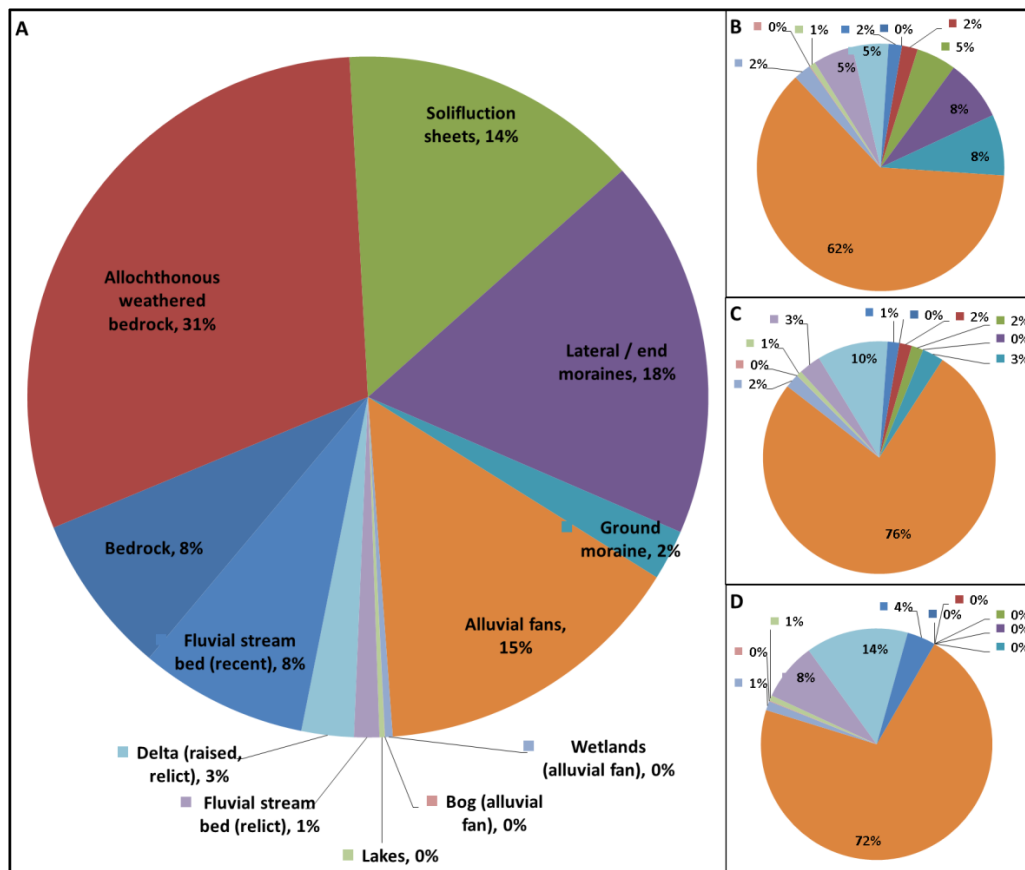
Figure 2. Proportional contribution of each landform to: A) Areal coverage of the total study area; B) total SOC storage for 0–100 cm; C) total SOC storage for 100–200 cm; and D) total SOC storage for 200–300 cm. Landform and colors from chart A apply also to charts B-D.
