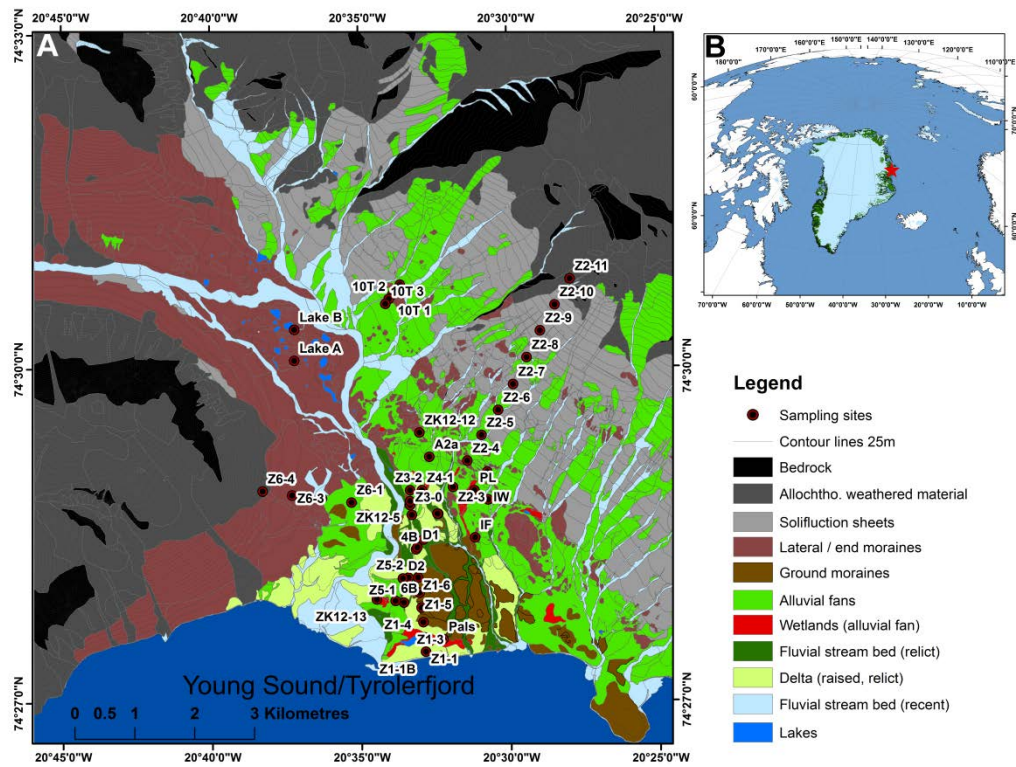
Figure 1. A) Simplified geomorphological landform map of the Zackenberg study area (based on Cable et al., 2017). B) Location of Zackenberg in NE Greenland.
