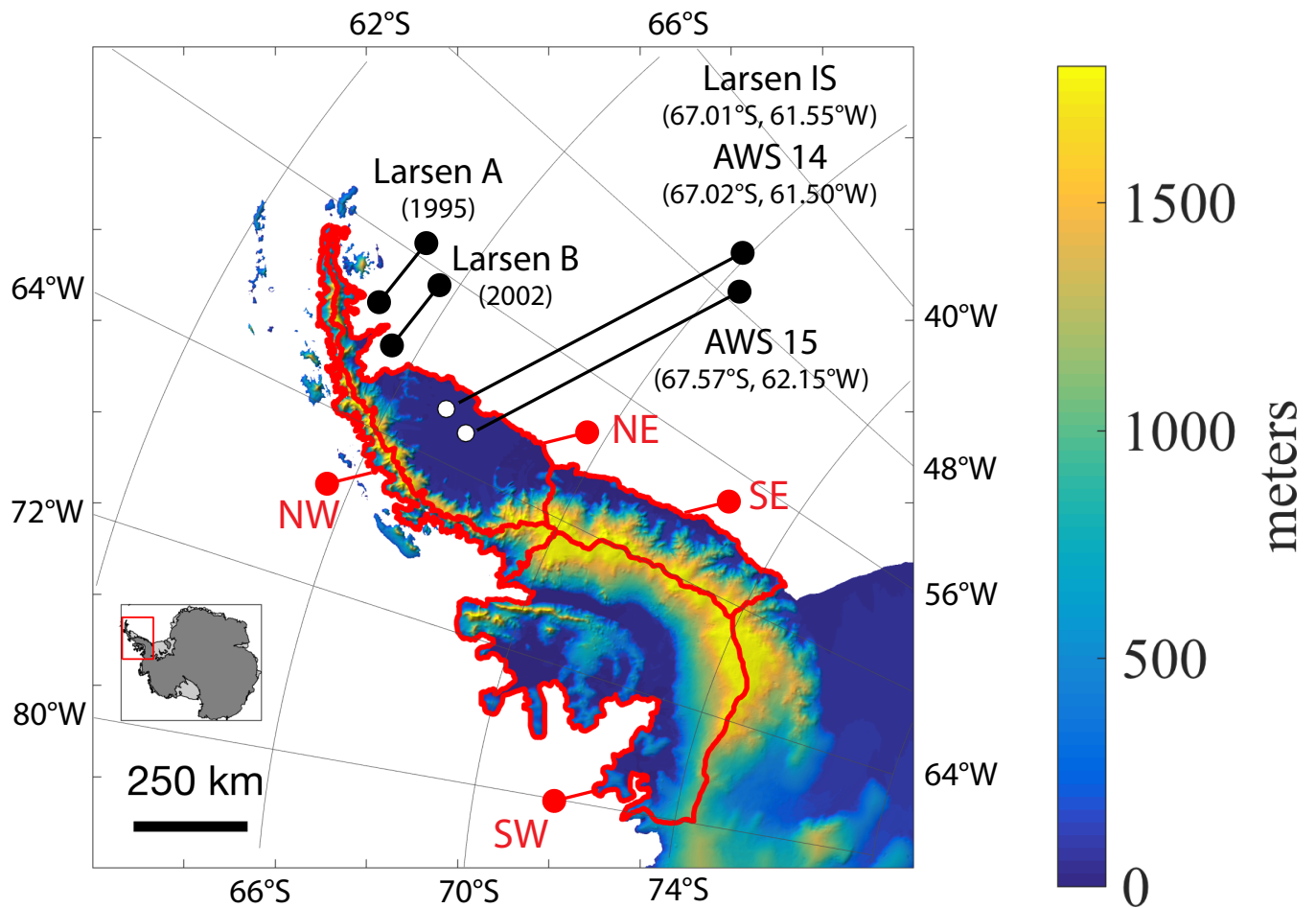
4 Figure 1: Full MAR domain showing topographic relief from bedmap2 ( https://www.bas.ac.uk/project/bedmap-2 ) at 1km, 5 former ice shelves with dates of collapse, locations of automatic weather stations (Larsen IS and AWS 14 stations are located 6 within the same MAR gridcell) and basins corresponding to SW (basin 24) NW (basin 25) NE (basin 26), SE (basin 27) 7 from Zwally,et. al. 2012
