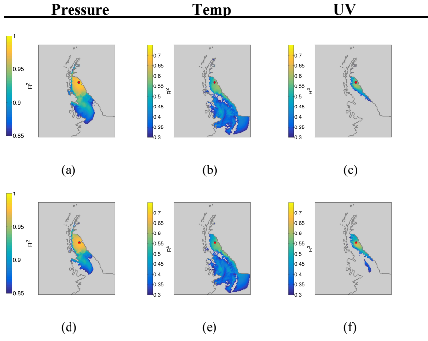
Figure S7: Left column is for surface pressure. Middle column for daily-averaged 2m air temperature, right column for 2m wind speed. Stations are as follows: (a)(b)(c) AWS 14/Larsen Ice Shelf, which are co-located in MAR (d)(e)(f) AWS 15
