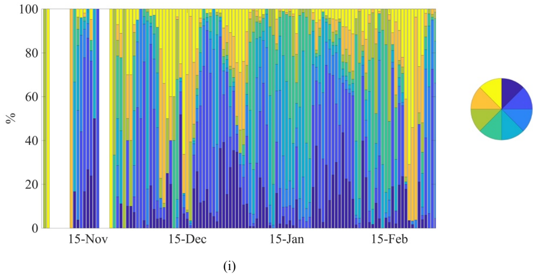
10 Figure S3 : Wind roses shown for the Larsen IS AWS station in 2001-2002 for (a)Nov (b)Dec (c) Jan (d) Feb. Wind roses 11 shown for the MAR grid cell co-located to the Larsen IS AWS station in 2001-2002 for (e) Nov (f)Dec (g) Jan (h) Feb.(i) 12 Proportion of wind direction (directions shown in inset) for all grid cells where MAR melt occurs in the NL region over the 13 melt season
