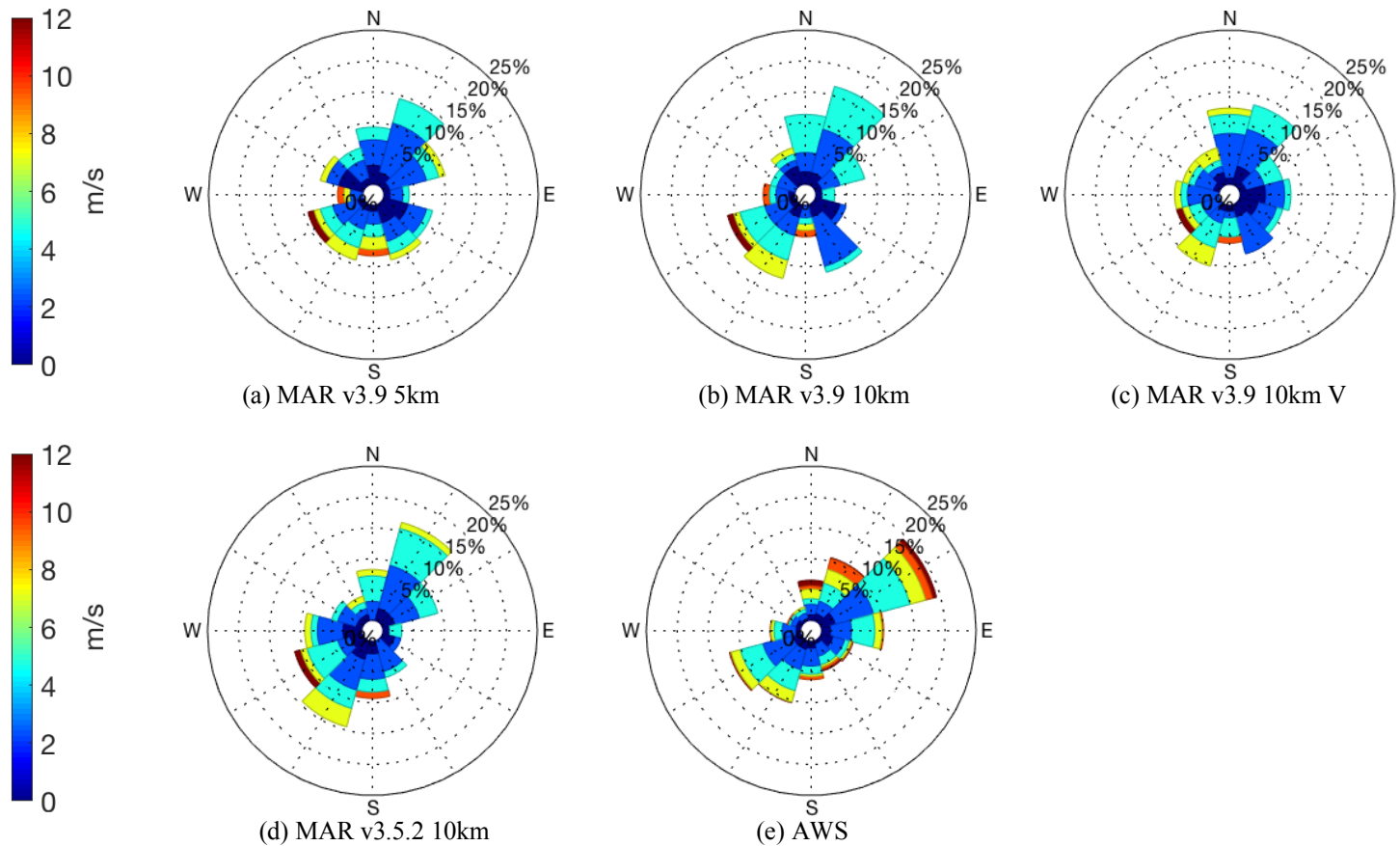
Figure S5: Wind roses at the Larsen IS AWS location (shown in Fig. 1) for Nov 1, 2004 – March 31, 2005 for MAR 3.9 at a 5km resolution, 23 sigma layers, daily values (a) 10 km and 23 sigma layers, daily values (b) 10km resolution and 32 sigma layers, daily values (c), MAR 3.5.2 at a 10km resolution and 23 sigma layers, daily values (d) and AWS at 3-hourly values (e). MAR values are calculated only when AWS data is available and AWS data reports no values between Dec 20, 2004 and February 12, 2005
