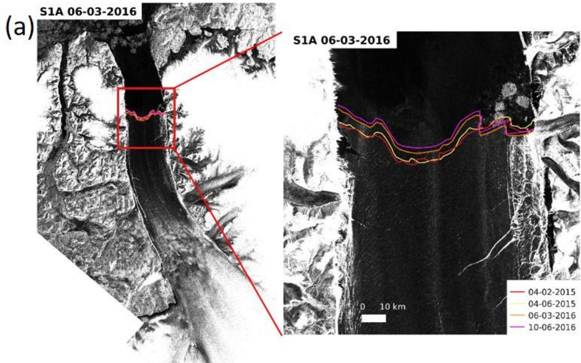
Figure S1: Ice front location extracted from Sentinel-1 images on (a) Petermann Glacier and (b) Nioghalvfjærdsfjorden.
