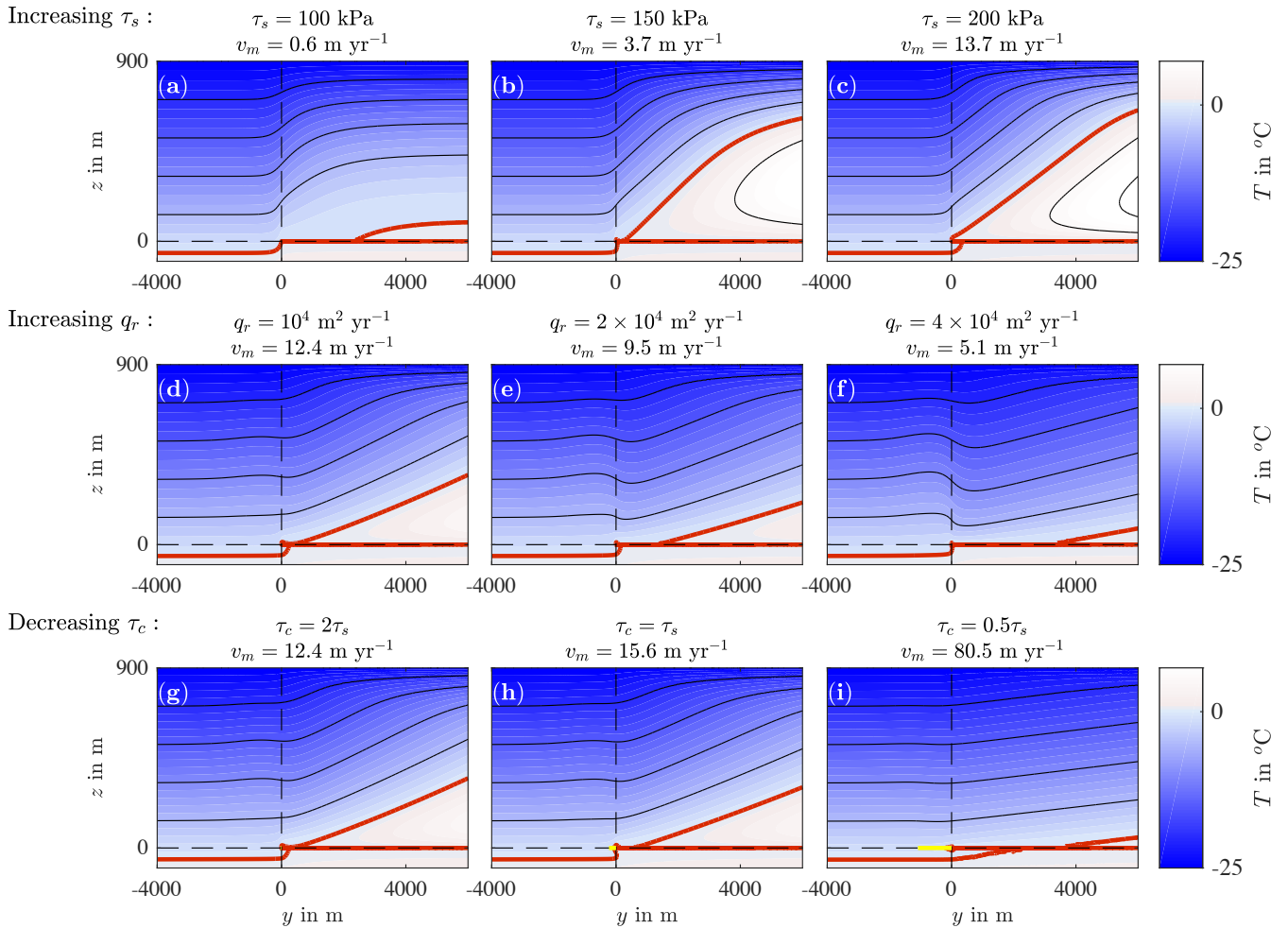
Figure 3. The effect of shear heating (represented by \tau_s ), advection (represented by q_r ), and subtemperate basal sliding (represented by \tau_c ) on the temperature field in an ice stream margin, same plotting scheme as in figure 2. Solid black lines show contours in 5^\circ\text{C} intervals with the contour of T = 0^\circ\text{C} in red. Thin dashed lines indicate the ice–bed interface and the location of the cold-temperate transition at the ice–bed interface. Red shading indicates the formation of temperate ice. Note that T should be interpreted as a proxy for moisture content when T > 0 . In this case we can identify \phi = \rho c_p T / (\rho_w L) with \phi the volumetric moisture content of the ice, \rho_w the density of water, and L latent heat per unit mass. Top row has q_r = 0 , \tau_c = \infty (i.e., no subtemperate slip), and values of \tau_s as indicated above the panel. Middle row has \tau_s = 200 kPa and \tau_c = \infty . Bottom row has \tau_s = 200 kPa and q_r = 10^4 m 2 year -1 . The yellow lines in panels g to i mark the extent of the subtemperate slip region. The far-field ice-ridge bed temperature was set to T_b = -10^\circ\text{C} to facilitate visualization, leading to relatively small migration velocities. All other values as listed in table 1.
