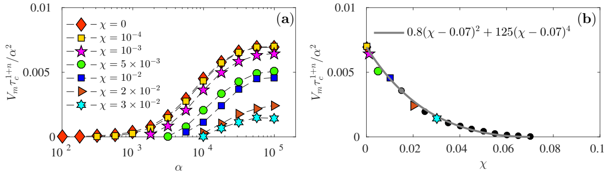
Figure 9. Asymptotic behavior for large \alpha and \text{Pe} for the case of intermediate slip ( 1 \ll \tau \lesssim \alpha^{1/(1+n)} ) where we expect a limiting behavior of V_m \tau_c^{1+n} \alpha^{-2} = g(\chi) , see (52). Panel a: V_m \tau_c^{1+n} / \alpha^2 against \alpha for different values of \chi = \tau_c^{1+n} \text{Pe}^{1/(1-\beta)} \alpha^{-2/(1-\beta)} with \text{Pe} fixed between 0 and 10^7 and \tau varying between 0.1 and 3.2. Convergence to constant values for \alpha \gg 1 confirms (52). Panel b: values of V_m \tau_c^{1+n} / \alpha^2 at different \chi for \alpha = 10^5 and \tau = 3.2 .
