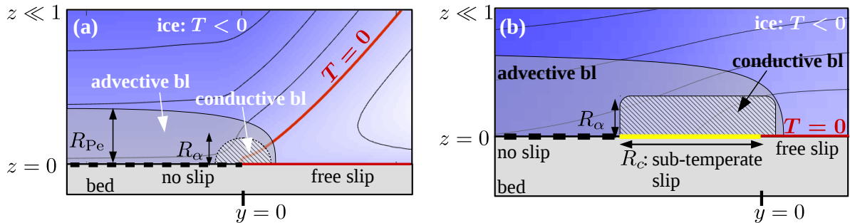
Figure 5. Boundary layer structure for asymptotics with large \alpha and \text{Pe} , without subtemperate slip (panel a ) and with subtemperate slip (panel b ). The background temperature profiles are enlargements of typical profiles in this asymptotic limit, with same color scale as in figure 3. In the outer advective boundary layer the temperature field close to the bed is advected from the ice ridge towards the inner conductive boundary layer. In case of a no slip/free slip transition at the bed the conductive boundary layer consists of a small region around the slip transition (panel a ). In case of subtemperate slip, the conductive boundary layer is a region of small vertical extent which stretches along the length of the subtemperate slip region (panel b ). Within the conductive boundary layer, heat dissipation is balanced by diffusion.
