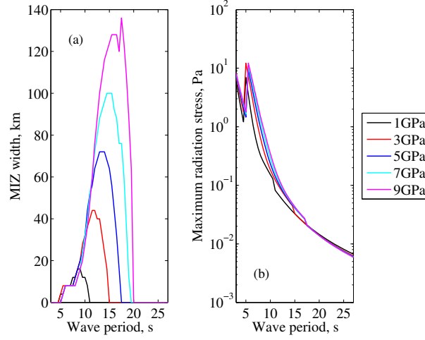
Figure 5. Variation of MIZ width (a) and maximum radiation stress (b) with peak wave period and Young's modulus for swells of height 3 m. The concentration was 0.7, the thickness was 1 m, and the small-scale cohesion used was 638 kPa. The WIM is not coupled to neXtSIM.
