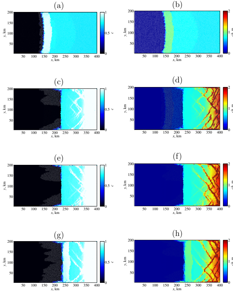
Figure 10. (a,b) Concentration ( c ) and effective thickness ( ch ) after the same experiment as Figure 7. (c,d) c and ch after forcing from uniform, steady wind. Same as Figure 1 (with speed 14.9\text{ms}^{-1} from the left) has been applied for 48h: wind forcing only. Figures (e–h) show results when steady waves (with H_s = 5 m, T_p = 11.2 s, from the left) are applied in addition to the wind forcing. Initial ice conditions are the same as in Figure 7. In (e,f) the ice rheology is not affected by the ice breakage, but in (g,h) damage is set to d_{\text{break}} = 0.9999 . The large-scale cohesion is \tau_0^L = 4 kPa, C = 40 , and the small-scale cohesion is \tau_0^S = 638573 kPa.
