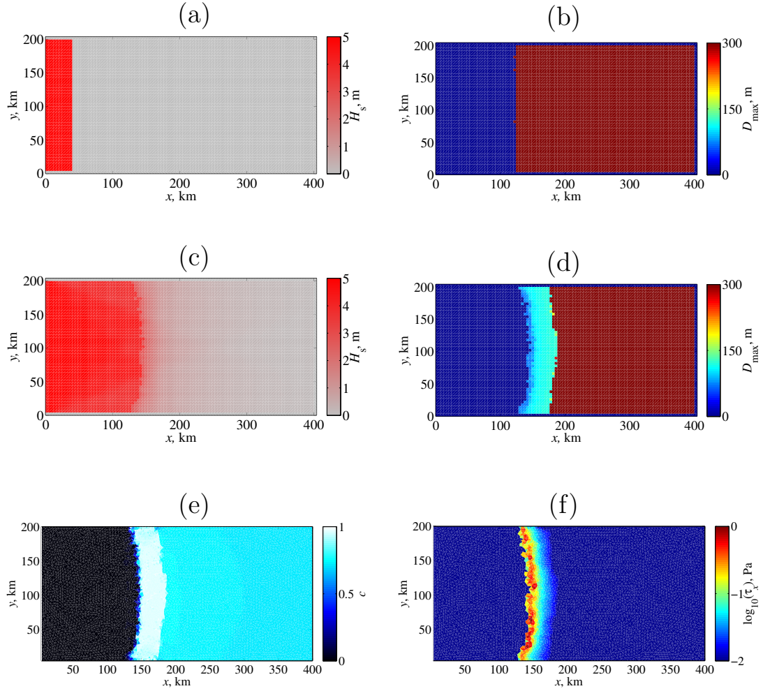
Figure 7. Waves breaking ice in an idealized experiment (the right hand, upper, lower lines of grid cells correspond to land). The wave model, based on (Williams et al. , 2013a), is coupled to the neXtSIM sea ice model. The figure shows results after 48 h of steady pushing by a Pierson-Moskowitz wind wave spectrum with significant wave height H_s = 5 m (so the peak period T_p = 11.2 s), that is arriving from the left. It initially occupies the strip shown in (a) then travels to the right, with some directional spreading; the final wave height is shown in (c). (b,d): initial, final maximum floe size (respectively); (e,f): final sea ice concentration and x -component of the wave radiation stress (respectively). The ice has initial conditions (constant where there is ice—see (b) for the initial ice mask): c = 0.7 , h = 1 m, D_{\max} = 300 m, and d = 0 . Also C=40 , \tau_0^L = 4 kPa, \tau_0^S = 638 \tau_0^S = 573 kPa, and d is increased to d_{\text{break}} = 0.9999 if the ice is broken.
