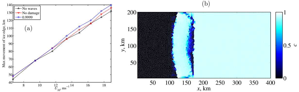
Figure 11. (a) shows the maximum movement of the ice edge as a function of wind speed. The different curves show the response to wind forcing only (“no waves”), wind and waves without changing the EB rheology in the MIZ (“no damage”), and wind and waves where the damage is set to d_{\text{break}} = 0.9999 in the MIZ (“0.9999”). (b) The effect of swell preconditioning on the response to off-ice winds. Initial conditions: swell of 12 s period and height 3 m is sent into the ice for 24 h, where the ice has constant concentration of 95% and thickness 1 m, breaking the ice for about 50 km. The damage is set to d_{\text{break}} = 0.9999 where the ice is broken. Spatially and temporally constant off-ice wind forcing is then applied for a further 48 h, at a speed of 2 \text{ m s}^{-1} . The large-scale cohesion is 13 kPa, and C = 40 .
