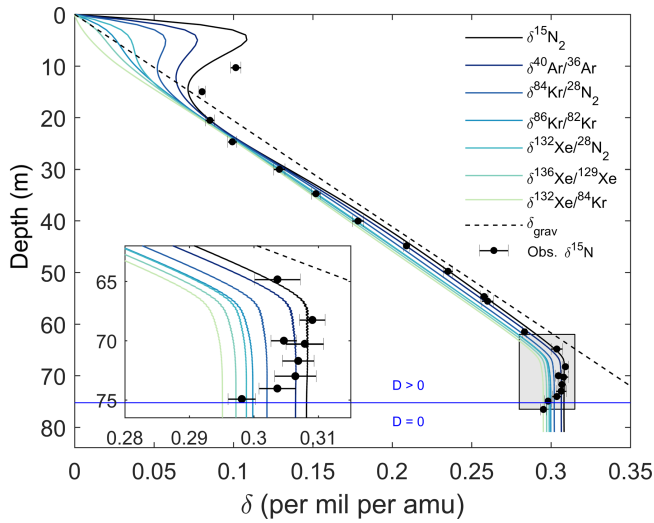
Figure 11. Horizontally averaged isotope ratios at WAIS Divide in the 2-D model including barometric pumping and horizontal layers. Isotope ratios are normalized to one atomic mass unit (amu) mass difference (Supplement). The dashed black line represents the equilibrium solution for pure gravitational settling ( \delta_{\text{grav}} ). The horizontal blue line marks the depth where vertical diffusivity reaches zero. Observed \delta^{15}\text{N} are shown as circles with horizontal error bars (Battle et al., 2011). The inset shows a magnification of the lock-in zone (gray patch).
