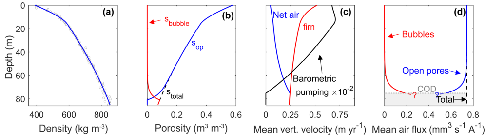
Figure 3. Firm conditions and modeled velocities profiles at WAIS Divide. (a) Density fit to observed data (data from Battle et al., 2011); (b) open, bubble (i.e., closed), and total porosity; (c) horizontally averaged barometric pumping velocity (i.e., time-mean horizontal average of |\mathbf{u}_b| , black), and horizontally averaged net air velocity ( \mathbf{w}_{\text{firm}} + \mathbf{w}_r , blue) and firm velocity ( \mathbf{w}_{\text{firm}} , red); (d) mean air flux in open pores (blue) and bubbles (red).
