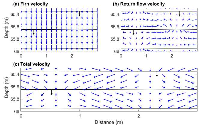
Figure 4. The different components of the velocity field: (a) firm velocity, (b) the velocity of air return flow to the atmosphere due to pore compression, and (c) net firm air advection velocity (a linear combination of the fields in panels a and b). Because of its alternating direction, barometric pumping yields no net flow but instantaneous flow field patterns look similar to panel (b). Black arrows indicate the downward advection of layers at the firm velocity.
