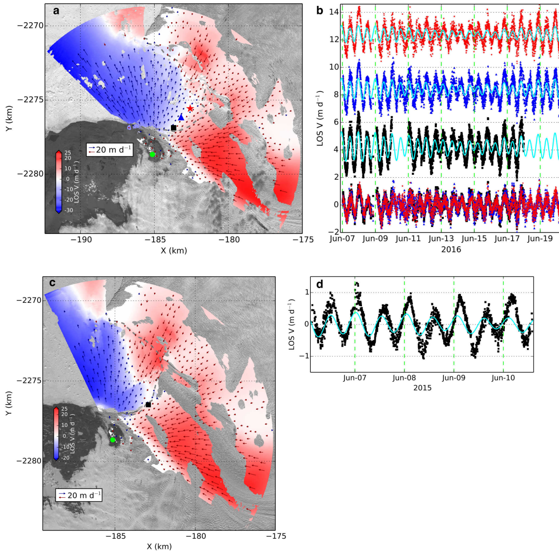
Figure 8. (a, b) Transverse-TRI observed non-parallel to long-term ice flow motion in the mélange of 2016. In (a), color map shows LOS velocity by interferometry, from a 1 day median average. Arrows show velocity estimates from feature tracking projected onto the LOS direction (dark red when ice moves towards the radar and dark blue when ice moves away). Dashed grey line shows eHff glacier front location from TRI image. black-Black square, blue triangle and red star mark three points where 2-D velocity direction is nearly perpendicular to radar LOS. Their LOS velocity time series are shown in (b). Note that the point with blue triangle marker corresponds to the marked point in Fig. 3(a). Top 3 rows in (b) show TRI observed LOS velocities for selected points; cyan curves are predicted LOS velocities based on the imaging geometry, assuming ice is free floating. LOS velocities are offset for clarity. Bottom row shows residual time series by subtracting the cyan curves. (c, d) Transverse-TRI observed non-parallel to long-term ice flow motion on the glacier front for 2015. Colors and arrows in (c) represent the same parameters as in (a). A point immediately adjacent to the eHff glacier front was chosen, marked by black square with its LOS velocity observed with TRI and predicted by tide variations shown in (d). Cyan curve in (d) shows predicted LOS velocities.
