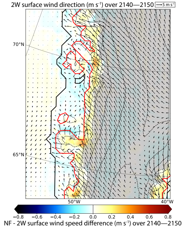
Figure 9. Surface wind speed difference (shaded) between the NF and the 2W experiments for the 2140—2150 mean period. Black arrows represent the wind direction in the 2140—2150 mean period of the 2W experiment. The length of the arrows indicate the magnitude of wind speed. The grey shaded area stands for the extent of the region for which the permanent ice fraction is 100 % (no tundra). Red solid line indicate the ice sheet extent The dashed black lines correspond to the 500 m surface elevation iso-contours.
