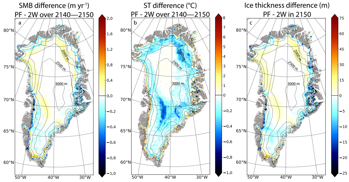
Figure 10. Mean differences (PF-2W) for the 2140—2150 mean period (a) Annual surface mass balance (in \text{m yr}^{-1} ) and (b) Annual surface temperature (in ^{\circ}\text{C} ) (c) ice thickness (in m) in 2150 between PF and 2W. Note that these differences are computed on the GRISLI grid. The dashed lines correspond to the 500 m surface elevation iso-contours of the present-day observed topography. The grey shade represents the non ice-covered areas.
