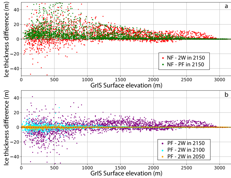
Figure 11. Ice thickness difference (m) as a function of the GrIS surface elevation (m) for the three coupling experiments. In (a) the red and green dots represent the NF-2W and the NF-2W differences in 2150; (b) Ice thickness difference (PF-2W) in 2050 (purple dots), 2100 (light blue dots) and 2150 (orange dots) mean periods.
