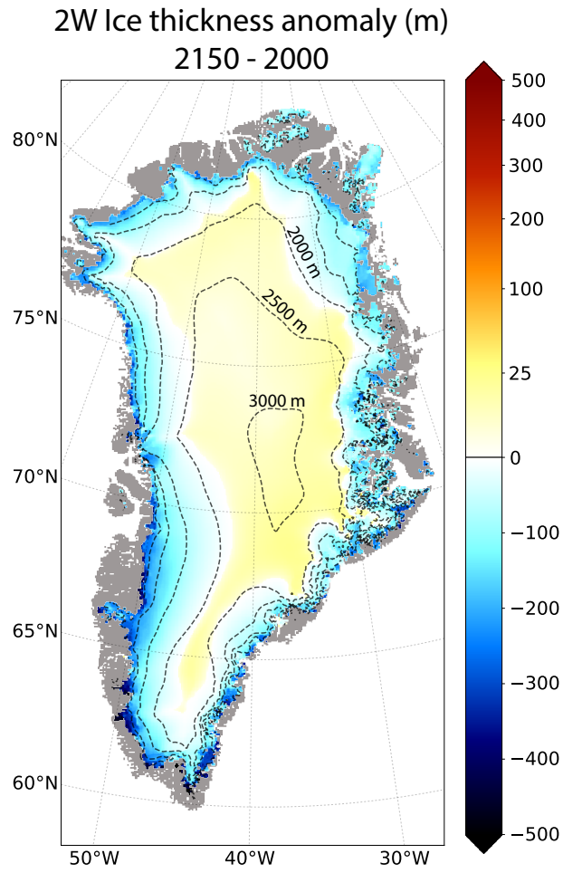
Figure 4. Ice thickness anomaly (2150-2000) simulated in the 2W experiment (in m). The dashed lines correspond to the 500 m surface elevation iso-contours for the present-day observed topography. The grey shade represents the non ice-covered areas. A non-linear color scale is used for positive values.
