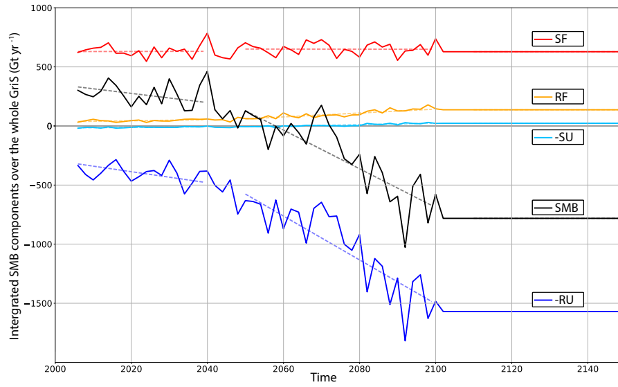
Figure 1. Evolution of the SMB (black line) and its components from 2005 to 2150 (in \text{Gt yr}^{-1} ) simulated by MAR in the 2W experiment and integrated over the ice sheet mask taken from Bamber et al. (2013). The SMB components are: snowfall (SF, red line), rainfall (RF, orange line), sublimation (-SU, light blue line), runoff (-RU, dark blue line). Dashed lines correspond to regression lines ranging from 2000 to 2039 and from 2041 to 2099. The light dark solid line corresponds to the zero line.
