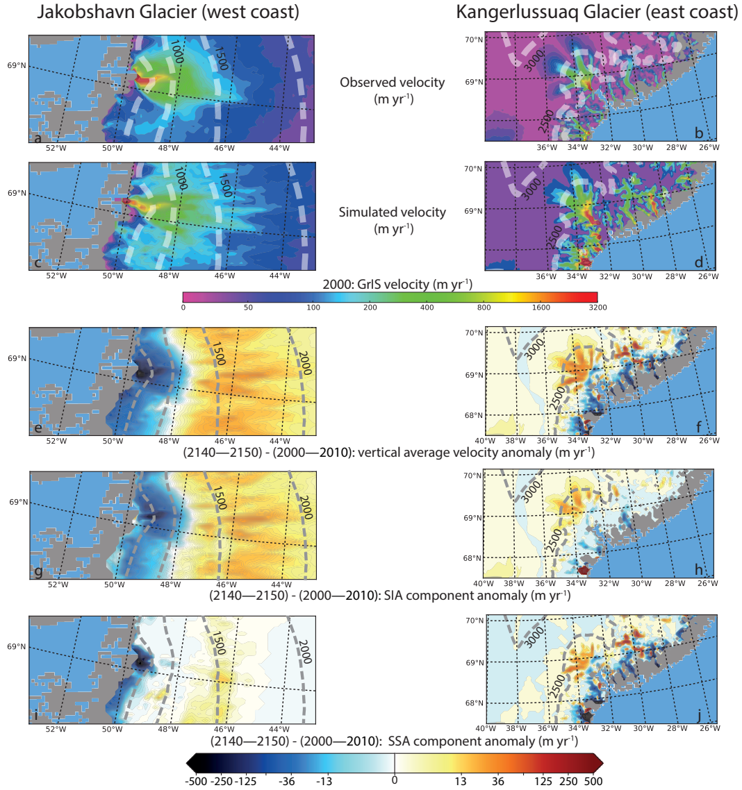
Figure 7. Regional zoom over the Jakobshavn (left panels) and the Kangerlussuaq (right panels) glaciers for the 2W experiment. (a) and (b) are the observed velocities (in \text{m yr}^{-1} ) from Joughin et al. (2018). (c) and (d) are the simulated velocity (in \text{m yr}^{-1} ) after the initialization procedure. Panels from (e) to (j) represent the velocity anomalies (in \text{m yr}^{-1} ) between the 2140—2150 and the 2000—2100 mean periods of the 2W experiment for the vertically averaged surface velocity (e and f), the SIA velocity component (g and h) and the SSA velocity component (i and j). Note that a logarithmic scale is used for the velocity anomalies. The dashed lines correspond to the 500 m surface elevation iso-contours for the present-day observed topography. The grey shade represents the non ice-covered areas and the blue shade is the ocean mask.
