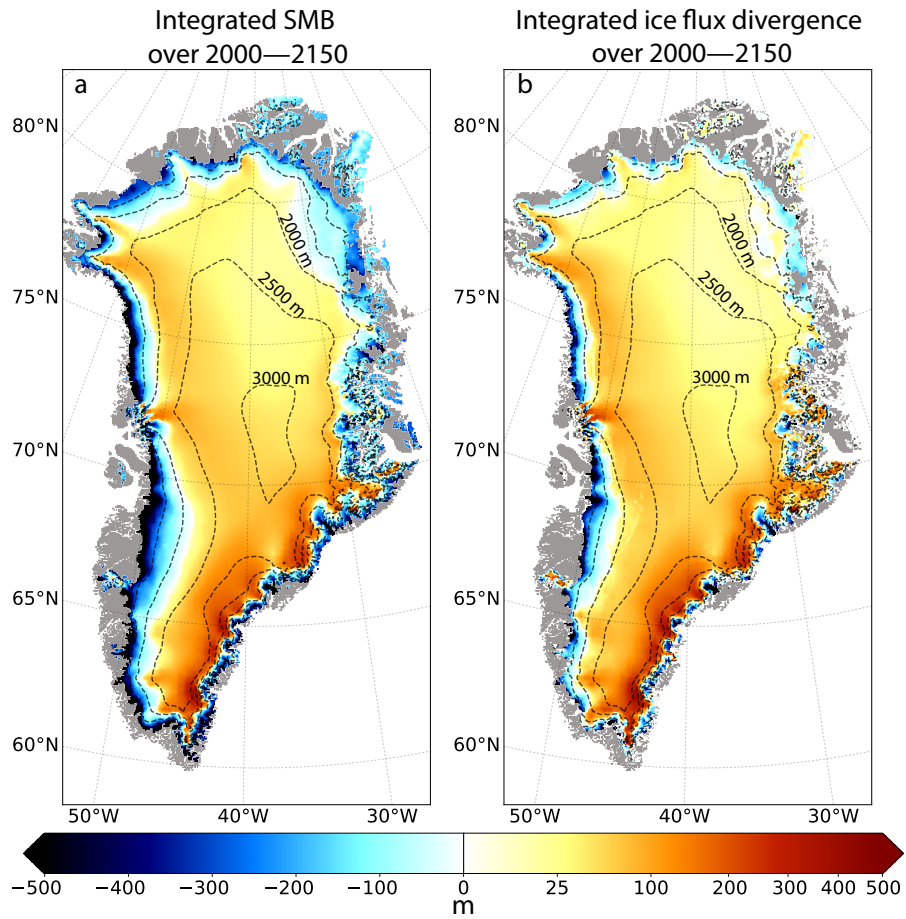
Figure 5. Cumulated SMB (a) and ice flux divergence (b) throughout the entire 2W experiment (from 2000 to 2150) given in meters and computed on the GRISLI grid. The dashed lines correspond to the 500 m surface elevation iso-contours for the present-day observed topography. The grey shade represents the non ice-covered areas. A non-linear color scale is used for positive values.
