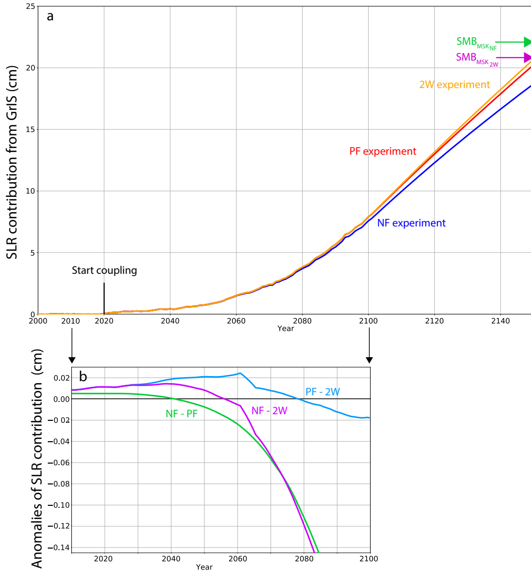
Figure 12. (a) Contribution of the GrIS to sea-level rise (in cm) as simulated in the NF (blue line), PF (red line) and 2W (yellow line) experiments and inferred from the ice thickness changes between the 2000 and 2150. Green and purple arrows indicate the projected contribution from GrIS inferred from SMB changes integrated over the same period over a fixed ice sheet mask ( SMB_{MSK_{NF}} ) and a time variable ice sheet mask ( SMB_{MSK_{2W}} ). (b) Zoom of the differences of GrIS contributions to sea-level rise between the PF and the NF experiments (green line), between the 2W and the NF experiments (purple line) and between the 2W and the PF experiments (light blue line).
