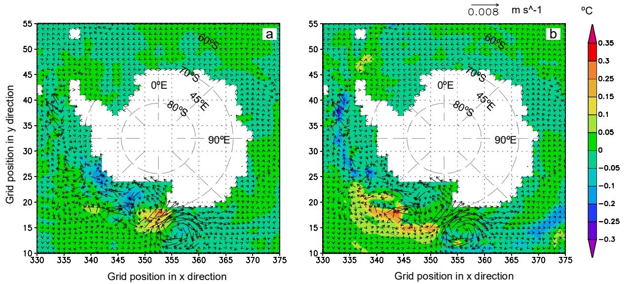
Fig. 6. Differences of sea surface temperature (shaded contours) and current (arrows) (EI minus EN). (a) March. (b) September. The units for temperature and current are ^{\circ}\text{C} and \text{m s}^{-1} , respectively.
