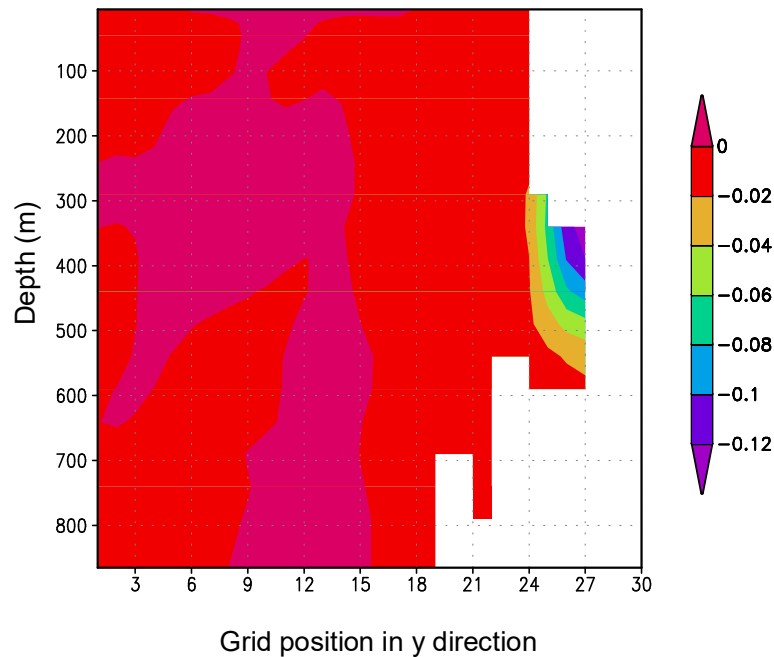
Fig. S3. Difference of density (EI-EN) in the cross-section along x=351 . The contour interval is 0.02 \text{ kg m}^{-3} .
