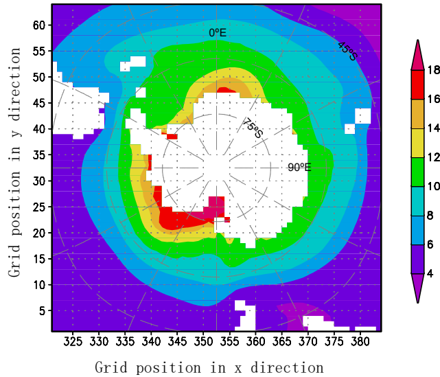
Fig. S2. Ratio of the coefficients of haline contraction and thermal expansion ( \beta/\alpha ) at 390 m in EN. The units of \beta and \alpha are \text{kg g}^{-1} and ^{\circ}\text{C}^{-1} respectively.
