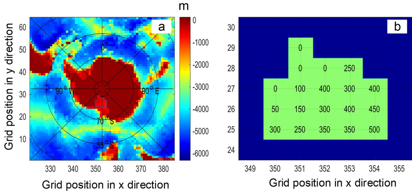
Fig. 1. (a) Bathymetry of the 6th cubed sphere face in the experiments and (b) cavity geometry of RIS in EI.
