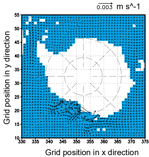
Fig. S4. Differences of annual mean ocean currents (EI minus EN) at 2065 m. The unit of velocity is m/s
