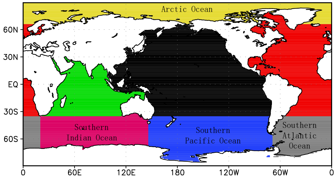
Fig. S1. Division of world ocean in 1 x 1 longitude-latitude grids
