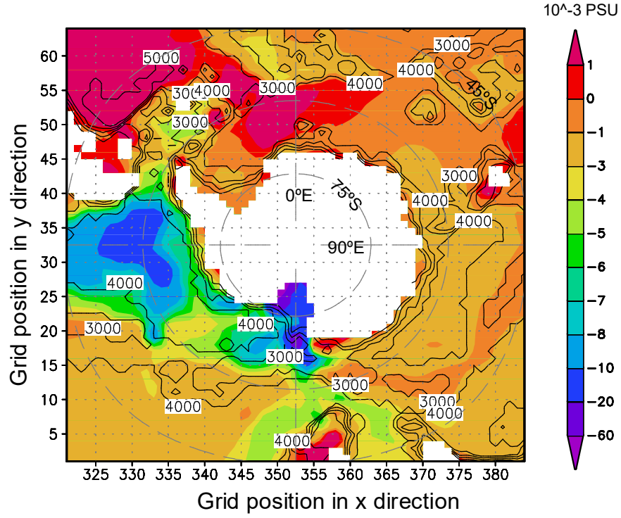
Fig. 5. Annual mean salinity differences (EI minus EN, shaded) at the sea bottom. The contour lines represent the water thickness with intervals of 1000 m. The unit for salinity is PSU.
