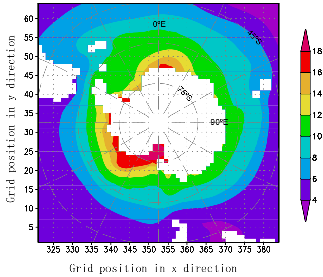
Figure S2. Ratio of the coefficients of haline contraction and thermal expansion ( \beta/\alpha ) at 390 m in EN. The units of \beta and \alpha are \text{kg g}^{-1} and ^{\circ}\text{C}^{-1} respectively.
