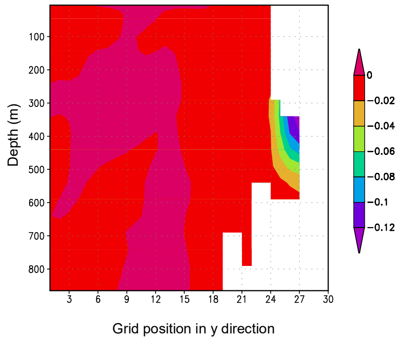
Figure S3. Difference of density (EI-EN) in the cross-section along x=351 . The contour interval is 0.02 \text{ kg m}^{-3} .
