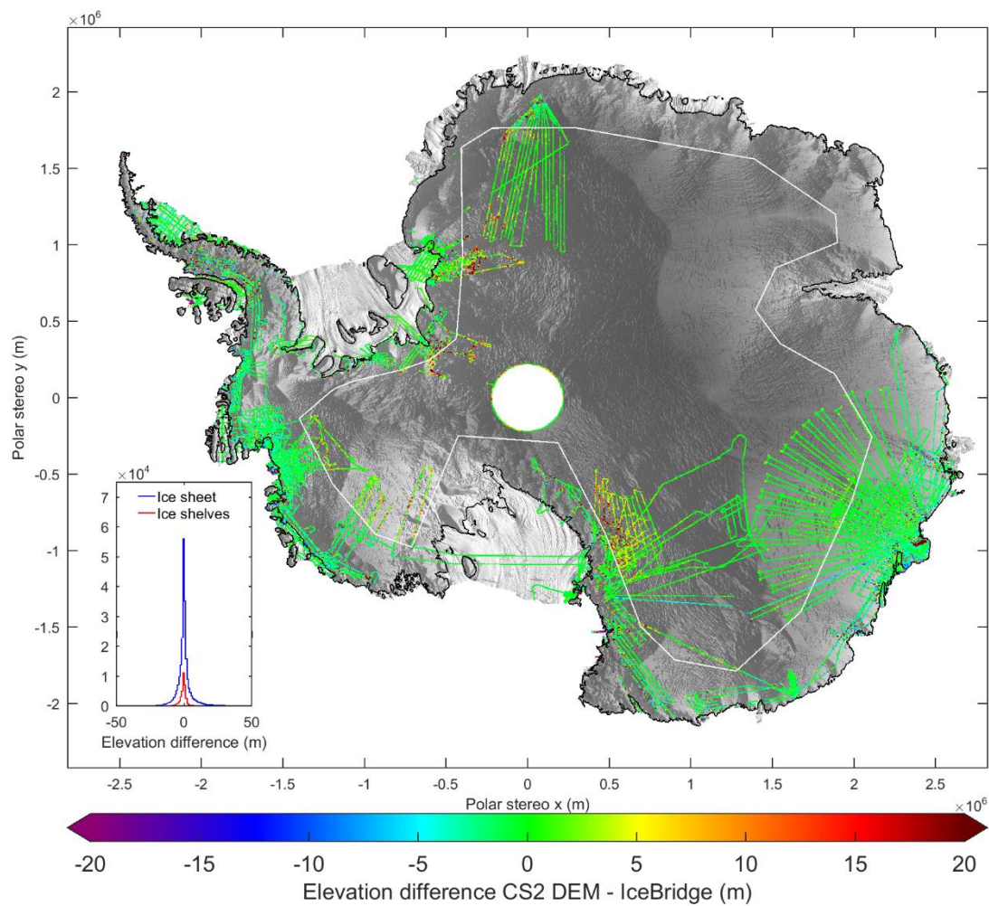
Figure 7: Difference between CryoSat-2 DEM elevation and airborne laser altimeter measurements in observed grid cells. Elevation differences are overlaid on a shaded relief plot of the DEM. (inset) Distribution of elevation differences (DEM – airborne) for the ice sheet and ice shelves.
