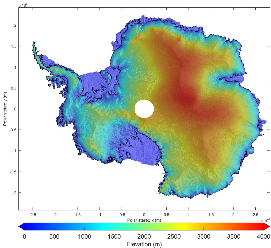
Figure 4: A new elevation model of Antarctica derived from 6 years of CryoSat-2 radar altimetry.
