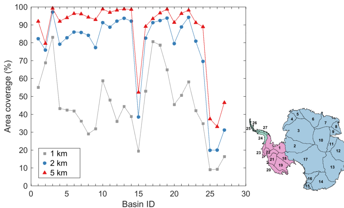
Figure 1: Area coverage of elevation values provided by the model fit solution of CryoSat-2 measurements for the Antarctic ice sheet, with a grid cell sizing of 1 km 2 , 2 km 2 and 5 km 2 . Solid black lines and numbers (inset) show the boundaries and ID numbers of the 27 drainage basins used (Zwally et al., 2012). East Antarctica and the Antarctic Peninsula are defined as numbers 2 to 17 and 24 to 27, respectively, and the remaining numbers define West Antarctica.
