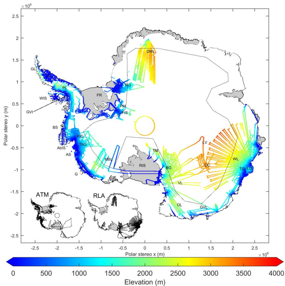
Figure 3: IceBridge airborne dataset used to evaluate the DEM, acquired between December 2008 and December 2014. The mode mask boundary (black) between CryoSat-2 LRM and SARIn modes is also shown. (inset) Locations of the individual ATM and RLA airborne datasets. Labelled are the following locations of interest: AbIS: Abbot Ice Shelf, AS: Amundsen Sea, BS: Bellingshausen Sea, BG: Byrd Glacier, DC: Dome C, DML: Dronning Maud Land, FIS: Foundation Ice Stream, FR: Filchner-Ronne Ice Shelf, G: Getz, GL: Graham Land, GVI: George VI Ice Shelf, GVL: George V Land, LC: Larsen-C Ice Shelf, LD: Law Dome, LV: Lake Vostok, MBL: Marie Byrd Land, OL: Oates Land, PIG: Pine Island Glacier, PL: Palmer Land, PM: Pensacola Mountains, RG: Recovery Glacier, RIS: Ross Ice Shelf, TG: Totten Glacier, ThG: Thwaites Glacier, TM: Transantarctic Mountains, VL: Victoria Land, WIS: Wilkins Ice Shelf, WL: Wilkes Land.
