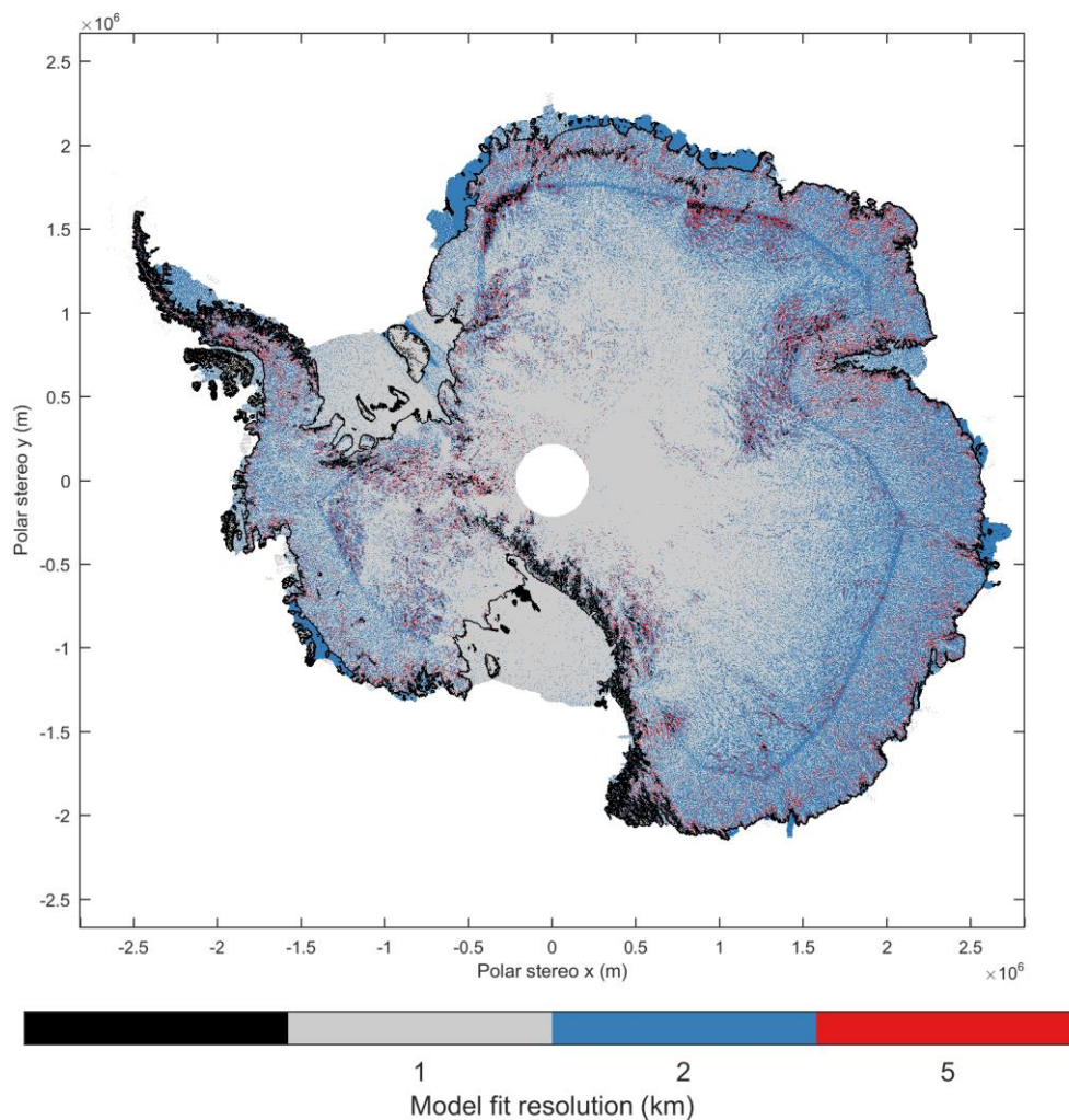
Figure 2: The grid cell resolution of the model fit method used to derive the surface elevation in each 1 km grid cell. Elevation values obtained from the 2 km and 5 km model fits are oversampled to the modal DEM resolution of 1 km. A black grid cell denotes a cell that contains an interpolated value. For the grounded ice sheet, approximately 60%, 30% and 5% of elevation values are derived from 1, 2 and 5 km model fits, respectively. For the ice shelves, 75% of elevations are calculated with 1 km model fits, and 23% from 2 km model fits. The remaining 5% of ice sheet and 2% of ice shelf values are interpolated using ordinary kriging.
