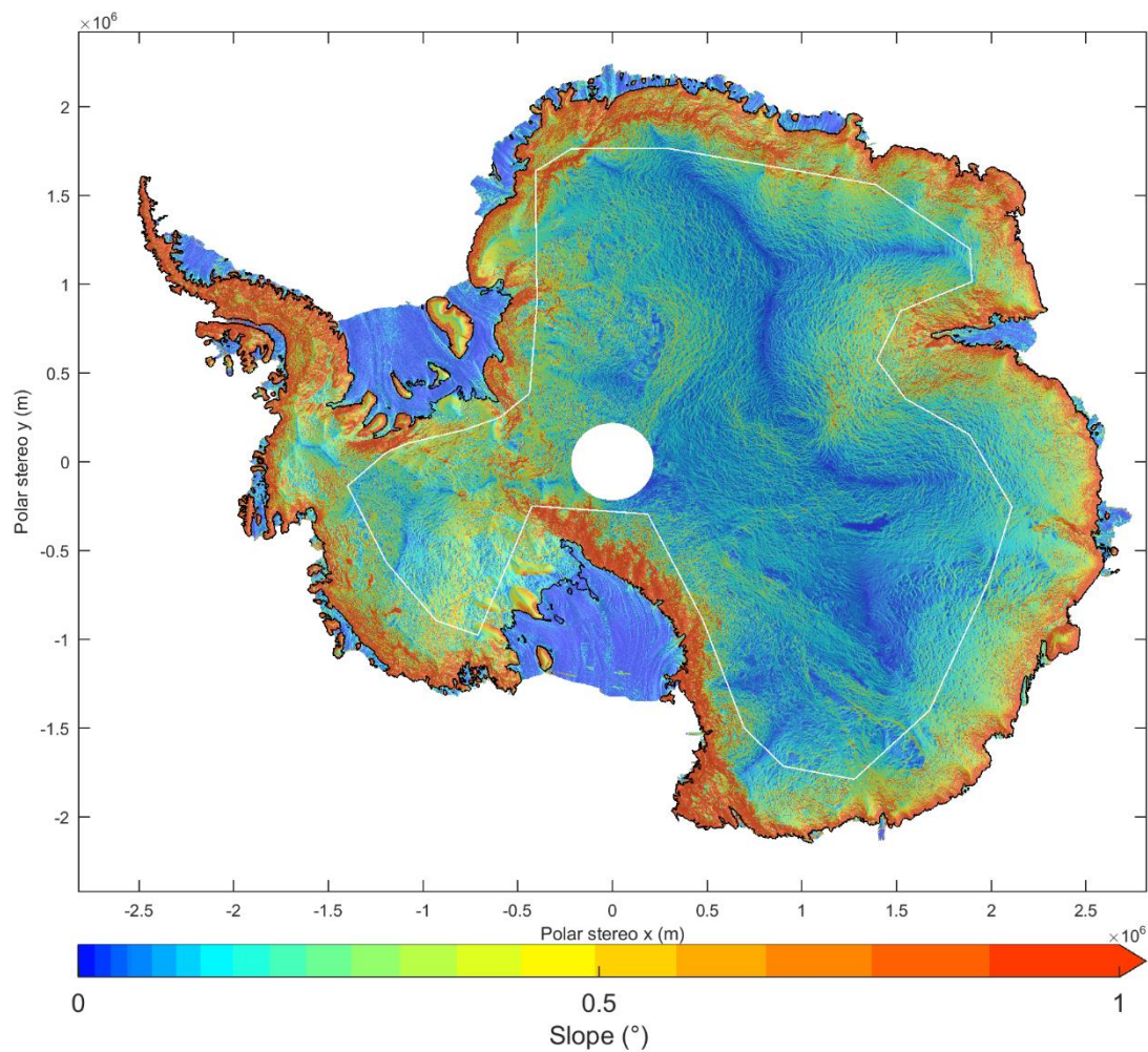
Figure 5: Surface slopes of Antarctica posted at a resolution of 1 km, derived from the digital elevation model. The mode mask boundary between CryoSat-2 LRM and SARIn modes is also shown in white.
