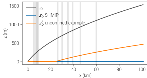
Figure 2. Experiments with artificial geometries. Vertical lines denote moulin positions for SHMIP/B2. The orange line shows the modified bedrock used to illustrate the impact of the confined/unconfined scheme as discussed in Sect. 3.2
