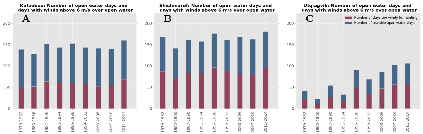
Figure 7. The number of days deemed too windy for boat travel for subsistence hunting ( > 6 m/s, (Ashjian et al, 2010)) are increasing along with the increasing number of open water days (number of days less than 15% sea ice concentration). Data taken from the WRF-downscaled ERA-Interim Reanalysis.
