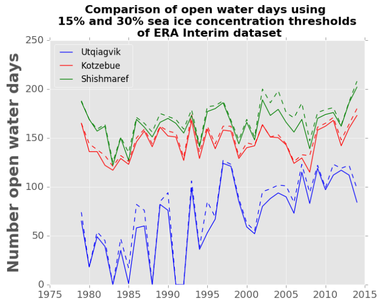
Figure 2. The number of open water days are similar if a 15% (solid line) or 30% (dashed line) sea ice concentration threshold is used. If the sea ice concentration (area of the grid cell) is lower than the threshold value, it is considered open water. Sea ice concentrations for the communities are extracted from the grid cells labelled as "Downscaled ERA" in Figure 1.
