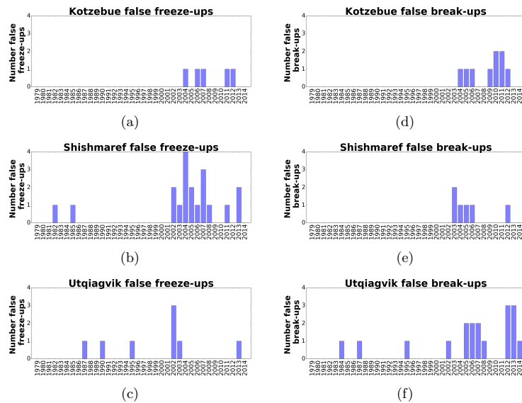
Figure 5: The number of false freeze-ups and break-ups per year, identified by ERA-I daily sea ice concentration data. False freeze(break)-ups are defined as the number of times the ice concentration oscillated above and below the sea ice concentration threshold value of 15% before the last freeze(break)-up was finally achieved.
