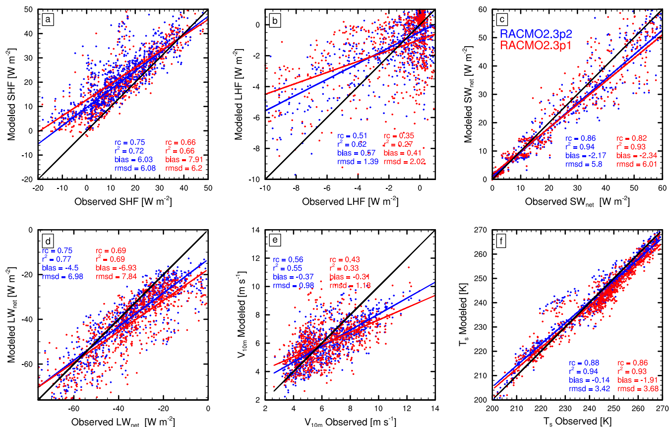
Figure 4. Correlation plots of RACMO2.3p2 (blue) and RACMO2.3p1 (red) as a function of the observation for (a) sensible heat flux (SHF), (b) latent heat flux (LHF), (c) SW net , (d) LW net , (e) V 10m and (f) T s . Denoted for all variables are the slope Rc, correlation coefficient r 2 , bias and root mean square deviation (RMSD) for both model versions.
