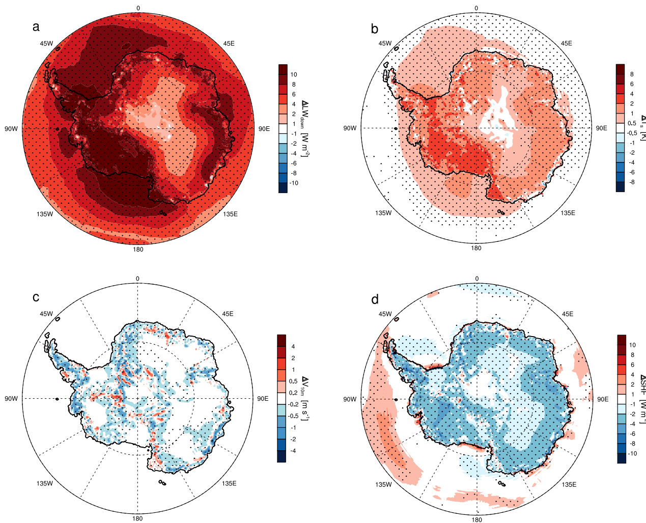
Figure 2. Annual average (1979–2014) difference (RACMO2.3p2 – RACMO2.3p1) of (a) downwelling longwave radiation ( LW_d ), (b) surface temperature ( T_s ), (c) 10 m wind speed ( V_{10m} ) and (d) sensible heat flux (SHF). Areas where the difference exceeds one unit of standard deviation of the difference are stippled.
