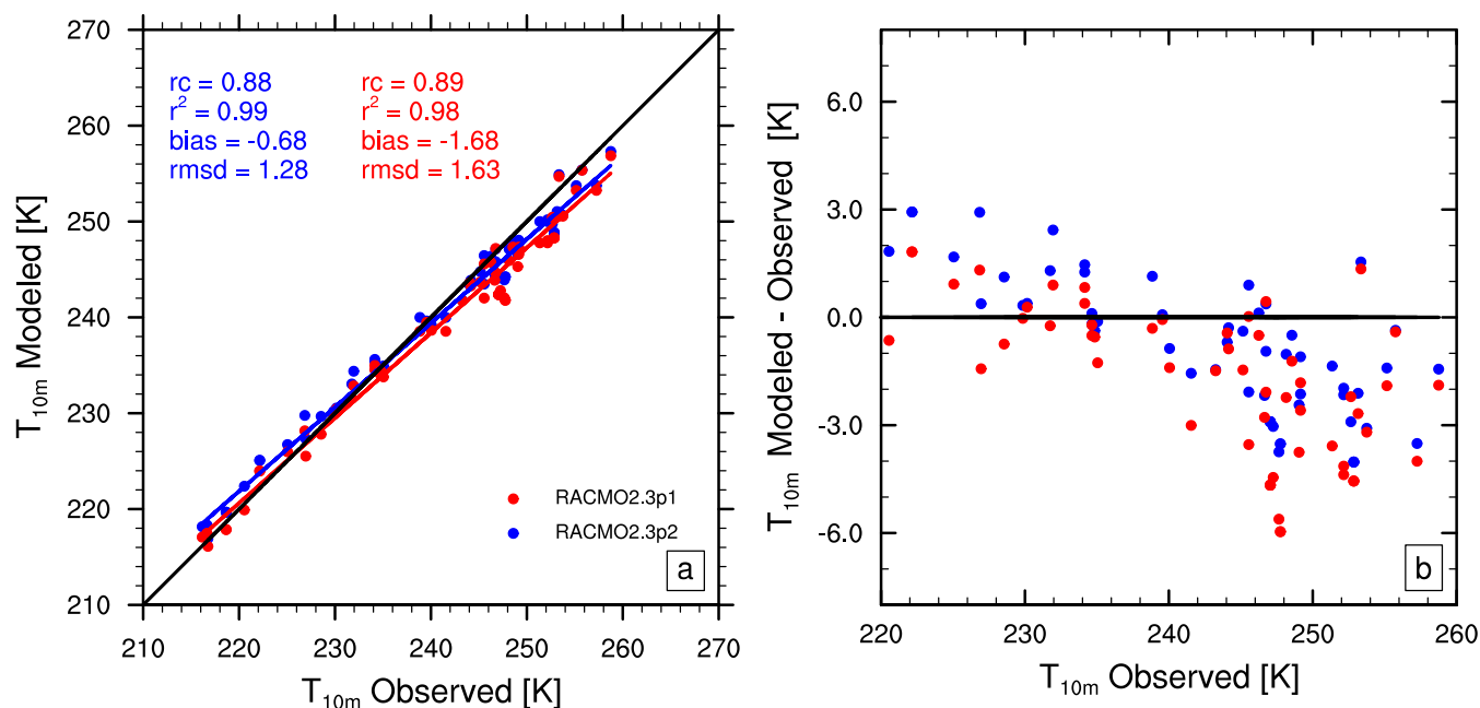
Figure 5. (a) RACMO2.3p2 (blue) and RACMO2.3p1 (red) and (b) modelled – observed 10 m snow temperature as a function of the 10 m snow temperature observations. Denoted are the slope, correlation coefficient r^2 , bias and root mean square deviation (RMSD) for both model versions.
