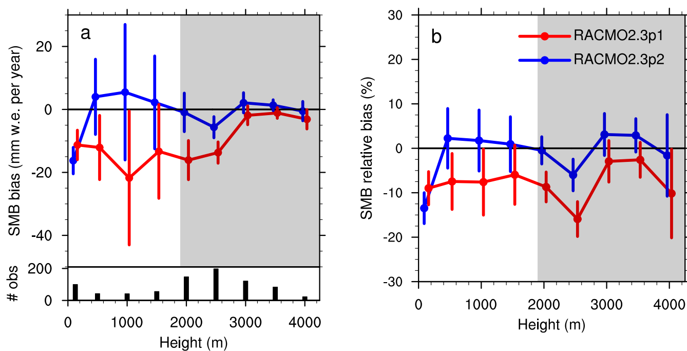
Figure 8. (a) Absolute bias and (b) relative bias ((\text{model} - \text{observation})/\text{model} \times 100\%) in modelled SMB for RACMO2.3p2 (blue) and RACMO2.3p1 (red). The data are binned in 500 m surface elevation intervals (0–250, 250–750, etc.). Error bars denote the combined uncertainty of the model and observations within each height bin, based on Van de Berg et al. (2006); Van Wessem et al. (2014a). Elevations above 2000 m (shaded grey) represent East Antarctica exclusively. The bar chart in (a) denotes the amount of weighted observations in each bin. To separate blue and red lines, x-axis locations of each bin are displaced by 75 m.
