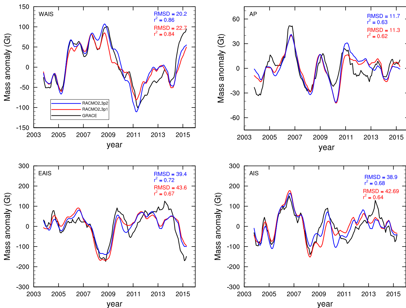
Figure 9. Detrended and deaccelerated average (for details see text) SMB anomalies of RACMO2.3p2 (blue), RACMO2.3p1 (red) and GRACE (black), release RL05, for West Antarctica (a), the Antarctic Peninsula (b), East Antarctica (c) and the whole Antarctic ice sheet (AIS, d). Shown are root mean square deviation (RMSD) and correlation ( r^2 ).
