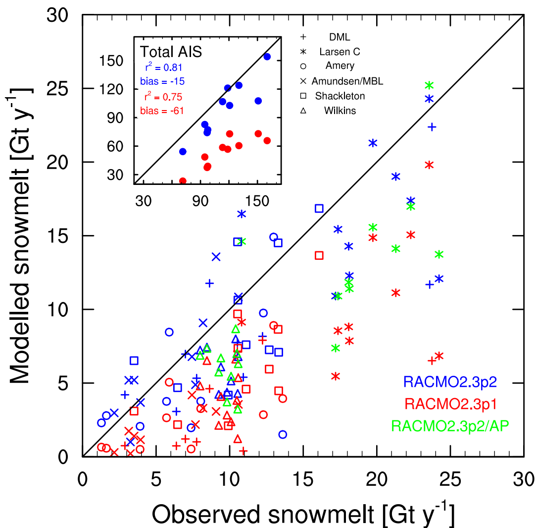
Figure 10. Modelled RACMO2.3p2 (blue), RACMO2.3p1 (red) and RACMO2.3p2/AP (green) as a function of observed QSCAT (Trusel et al., 2013) snowmelt in \text{Gt y}^{-1} . Shown are yearly 2000-2009 values for the total AIS (subpanel) and area averaged values for six regions in Antarctica defined in Trusel et al. (2013): Dronning Maud Land (DML, plus signs), Larsen C ice shelf (asterisks), Amery Ice Shelf (open circles), Amundsen/Marie Byrd Land (crosses), Shackleton Shelf (squares) and Wilkins Ice Shelf (triangles). Denoted are correlation r^2 and bias for the total AIS.
