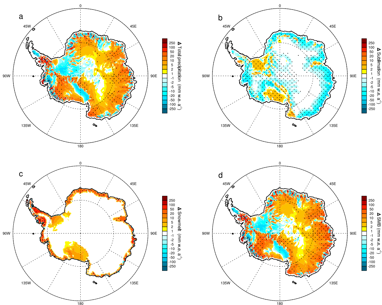
Figure 3. Annual average (1979–2014) difference (RACMO2.3p2 – RACMO2.3p1) of (a) total precipitation (snow + rain), (b) total drifting (snow + surface) sublimation, (c) snowmelt and (d) SMB. Areas where the difference exceeds one unit of standard deviation of the difference are stippled.
