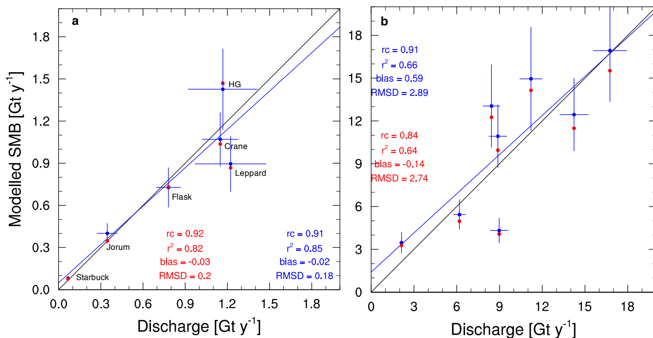
Figure 12. Modelled RACMO2.3p2/AP (blue) and RACMO2.3p1/AP (red) integrated average (1979–2016) SMB as a function of glacial discharge estimates from (a) the Larsen B embayment (Wuite et al., 2015) and (b) the George VI embayment (Hogg et al., 2017). Horizontal error bars represent the uncertainty in the discharge estimate, vertical bars the interannual variability of RACMO2.3.
