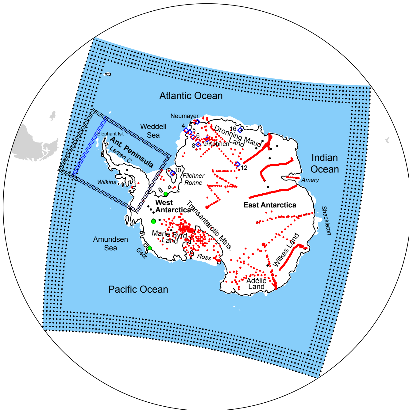
Figure 1. Map of Antarctica showing the in-situ SMB observations (red dots), AWSs (blue diamonds), the three snow radar regions (green dots), 64 10 m snow temperature observations (black dots) used in this study. Shown are the relaxation zones for both RACMO2.3p2/ANT and RACMO2.3p2/AP with the black dotted rectangles, as well as the RACMO2.3p1/AP domain (blue rectangle for the non-overlapping boundary). Also shown are the grounding line in black and relevant locations as used throughout the text (with ice shelves in italics).
