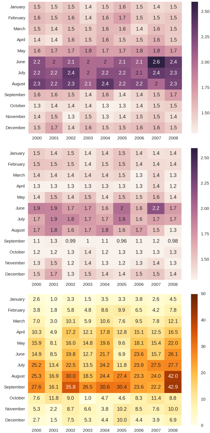
Figure 6. Sum of the sea ice area root-mean-square error (RMSE) (compared to assimilated sea ice at every grid location) for every month (in 10^6 km 2 ), before assimilation (top), after assimilation (middle) and the percent difference between the two (bottom). Positive differences correspond to a decrease of the RMSE and vice-versa.
