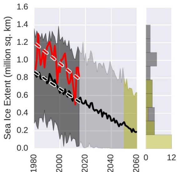
815 Figure 13: Observed (red line) September sea ice extent over Canadian marine regions ( SIC > 0.15 ); CMIP-5 multi-model mean (black line) and spread (shading). Histogram on the right shows the model distribution for 1980-2015 in black and for 2050-2060 in yellow.
