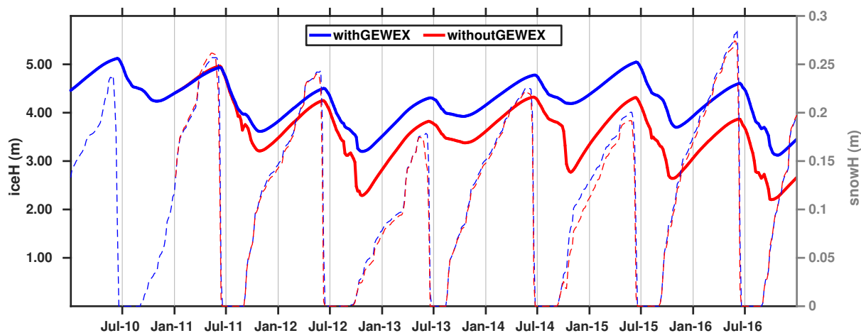
Figure 18. Simulated ice thickness (solid lines, left y-axis, unit: meters) and snow depth (dashed lines, right y-axis, unit: meters) at WEU Eureka in an ANHA4-CGRF simulation with GEWEX (blue) and without GEWEX (red) radiation flux correction
