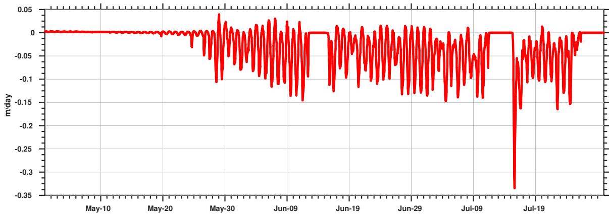
Figure 10. Diurnal cycle of thermodynamic ice production (unit: \text{m/day} ) during the break-up season at YCBB Cambridge Bay.
