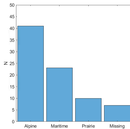
5 Figure 4. Snow climate classes for 81 FOCUS stations.
