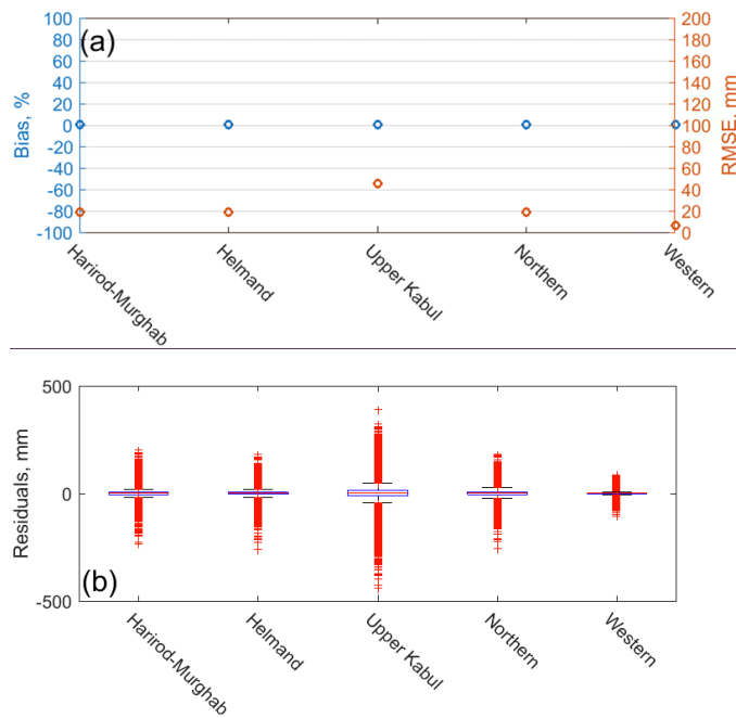
Figure 9. Same as Figure 8 except by basin for all years, (a) Bagged trees bias and RMSE; and (b) residuals.
