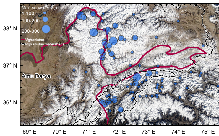
Figure 3. Maximum snow depth from WY 2017 manual measurements at FOCUS stations in Afghanistan, Pakistan, and Tajikistan overlaid on a MODIS true color image.
