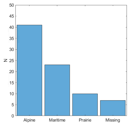
Figure 4. Snow climate classes for 81 FOCUS stations.
