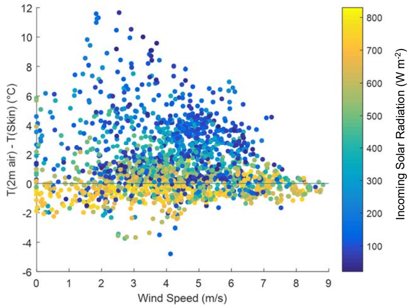
Figure 6: Difference between 2m air temperature and IR skin temperature showing the presence of strong surface-based inversions at low wind speeds and low values of incoming solar radiation (indicated by the marker colour).
