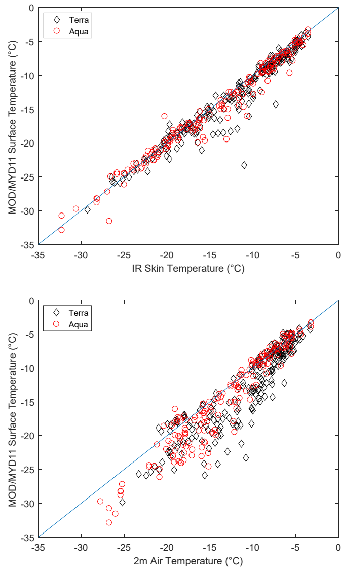
600 Figure 8: a) Direct comparison of in situ IR skin temperature data with MOD/MYD11 C6 surface temperatures. Agreement between satellite and ground-based measurements is quite good (RMSE = 1.6°C, n=374), and there is not a noticeable difference between the performance of the MOD11 and MYD11 temperature products, on the Terra and Aqua satellites, respectively. b) Direct comparison of 2 m air temperature with MOD/MYD C6 surface temperatures. This is illustrative of bias that may be inferred if 2 m air temperature is used in validation studies when inversions are present. RMSE = 3.1°C.
