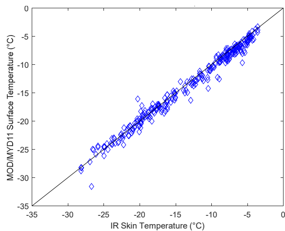
Figure 10: Comparison of MOD/MYD11 to in situ IR skin temperature after cloud-affected data are removed. The RMSE is 1.0°C and the mean bias is -0.4°C.
