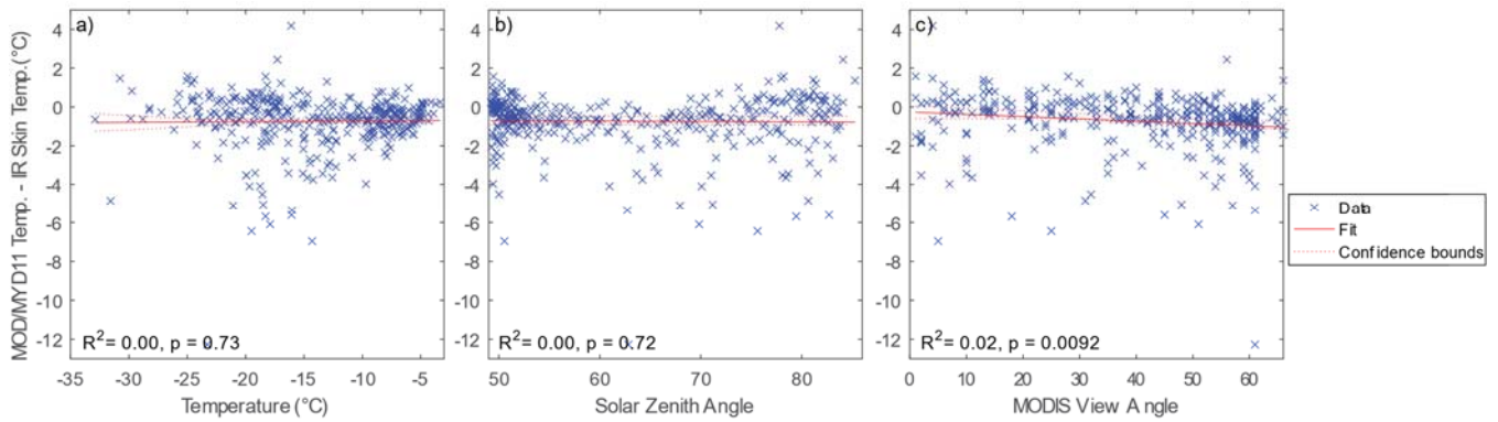
Figure 9: Difference in temperature measured from MOD/MYD11 and in situ IR skin temperature measurements as a function of a) IR skin temperature, b) solar zenith angle, and c) MODIS viewing angle. The only significant relationship is that the temperature difference is sensitive to the MODIS viewing angle. While the relationship is statistically significant, it is not a strong control on the temperature difference.
