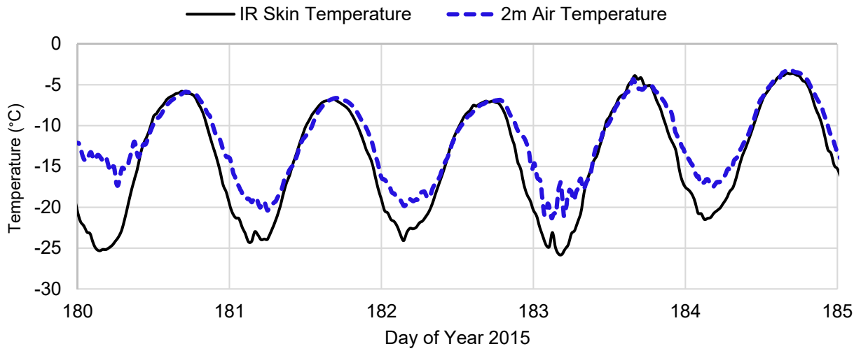
570 Figure 4: Time series of IR skin temperature, 2 m air temperature, during a clear sky period near Summit, Greenland.
