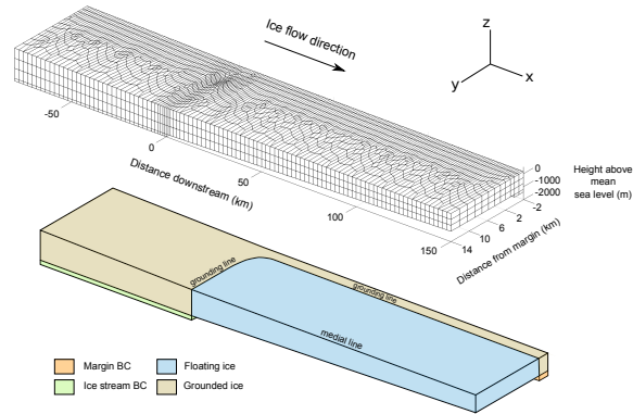
Figure 3. Finite element mesh used in the full-Stokes viscoelastic model (Sect. 4). Note that x and y horizontal scales have been reduced by factor 10 and 2 respectively.
