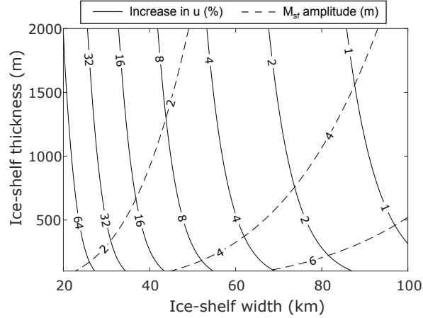
Figure 2. Contour plot of ice-shelf speed up due to tides, as a percent of the baseline speed, predicted by the analytical solution in Eq. 18. Speed-up is predicted along the ice shelf medial line using parameter values given in Table ???. Also shown are contours of the amplitude of the M_{sf} signal in ice-shelf displacements (dashed contours).
