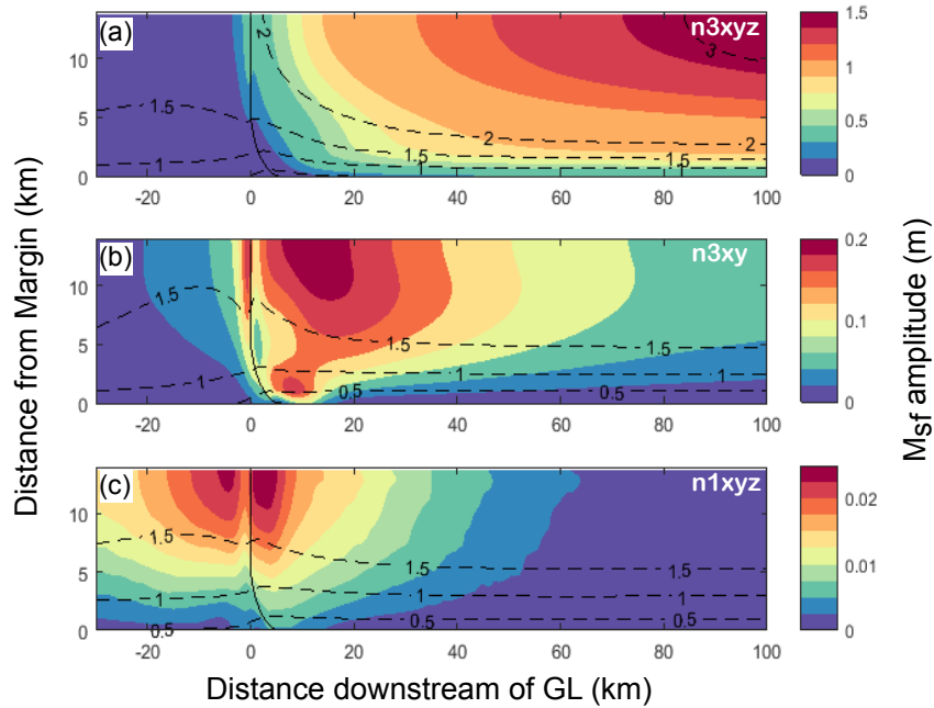
Figure 4. Plan view of M_{sf} amplitude in horizontal surface ice displacements, calculated with the full-Stokes viscoelastic model for the three experiments described in Section 5. Panel a shows experiment n3xyz , i.e. the standard case with n = 3 and bending all along the sidewall boundary. Panel b shows experiment n3xy in which the ice only bends at the x = 0 GL. Panel c shows the n1xyz experiment, for which n = 1 but with the same BCs as panel a. Dashed black lines are contours of downstream mean surface ice velocity and solid black lines show the GL position. Note the differences in colour scale between each panel.
