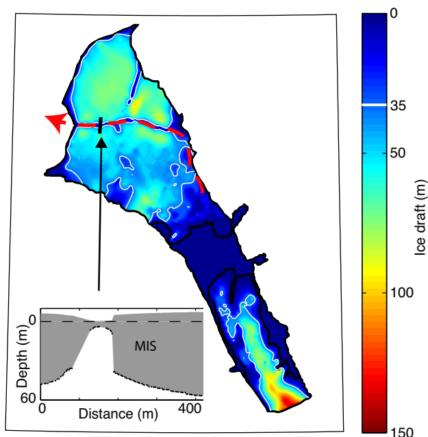
Figure 3. Map of the draft of ice in Milne Fiord indicating the likely drainage pathway of the MEL along a re-healed fracture in the MIS. The modelled ice draft is that presented in Hamilton (2016) from ground-based, aerial, and satellite ice thickness and surface elevation data assuming the ice is in hydrostatic equilibrium. The 35 m contour is highlighted to show the outflow restriction the MIS imposes across the mouth of the fjord for water above this level. The inset shows ice thickness across the basal channel from a 400 m ice-penetrating radar transect that crossed the re-healed fracture in July 2013 (Hamilton, 2016).
