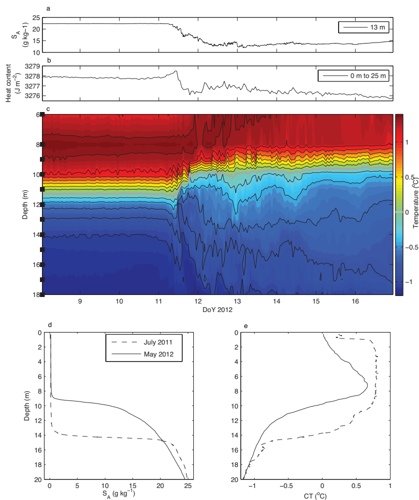
Figure 8. January 2012 MEL halocline mixing event. Time series of (a) salinity at 13 m depth, and (b) heat content between 0 m and 25 m, (c) temperature between 6 m and 18 m depth. The isotherm increment is 0.2^{\circ}\text{C} and the 0^{\circ}\text{C} isotherm (gray) is highlighted as a proxy for the bottom of the epishelf lake. Black squares on y-axis indicate the depths of thermistors. Profiles of (d) salinity and (e) temperature from field campaigns 6 months before (July 2011) and 4 months after (May 2012) the mixing event show the permanent change in the structure of the halocline (note that some of the change in the depth of the halocline is due to seasonal processes).
