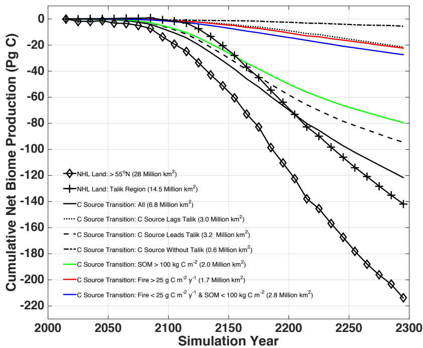
Fig. 3. Figure 8. Cumulative net biome production (NBP) over northern high latitude (NHL) regions (> 55°N) from 2010 to 2300. NBP < 0 represents a net C source. NHL regions are divided into the following categories
