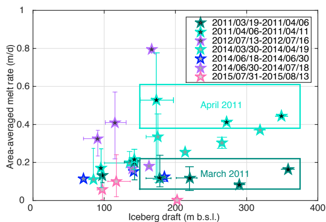
Figure 5: Area-averaged submarine melt rates plotted against median draft for icebergs calved from Jakobshavn Isbræ, west Greenland, into Ilulissat Isfjord. As in Figure 4, the symbols mark the median values and the error bars mark the range of estimates for each draft bin. The face colors and edge colors of the symbols indicate the year and month of the observations, respectively, as described in the legend. Deep melt rate estimates for the time period of rapid, significant change are circled for emphasis.
