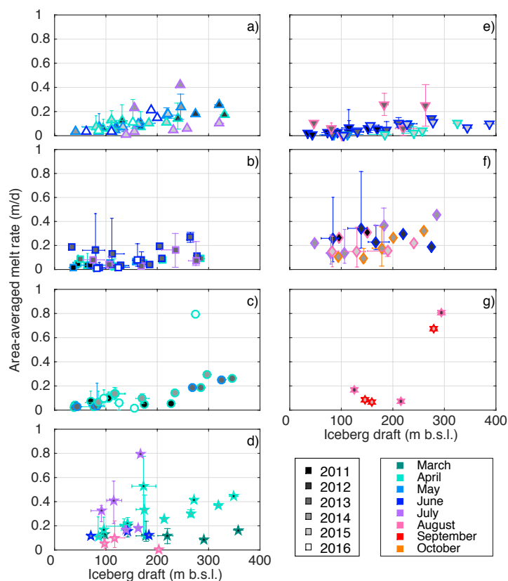
Figure 4: Area-averaged iceberg melt rate (meters per day) plotted against median draft (meters below sea level) for icebergs sampled near the terminus of (a) Kong Oscar Glacier, (b) Alison Glacier, (c) Upernavik Glacier, (d) Jakobshavn Isbræ, (e) Zachariae Isstrøm, (f) Helheim Glacier, and (g) Koge Bugt Glacier. For each observation period, icebergs were organized into 50 m-deep draft bins and the median melt rate and draft were computed. The symbols mark the median values and the error bars mark the range of estimates for each draft bin. The face colors and edge colors of the symbols indicate the year and month of the observations, respectively (see legends).
