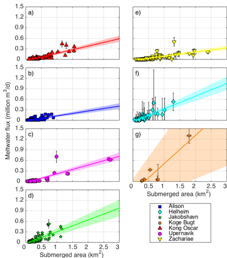
Figure 2: Liquid freshwater fluxes (millions of cubic meters per day) plotted against the estimated submerged area (square kilometers) for all icebergs sampled near the terminus of (a) Kong Oscar Glacier, (b) Alison Glacier, (c) Upernavik Glacier, (d) Jakobshavn Isbræ, (e) Zachariae Isstrøm, (f) Helheim Glacier, and (g) Koge Bugt Glacier. Vertical error bars indicate the meltwater flux uncertainties due to random DEM errors, ice density uncertainties, surface meltwater flux uncertainties, and manual iceberg delineation errors. Horizontal error bars indicate the range of submerged iceberg areas predicted for cylindrical submerged geometries using surface elevation and map-view surface area estimates extracted from repeat DEMs. Linear polynomials fit to the datasets compiled for each study site are plotted as thick colored lines and the surrounding shaded envelopes encompass their 95% confidence intervals.
