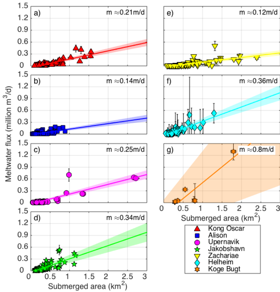
5 Figure 2: Liquid freshwater fluxes (millions of cubic meters per day) plotted against the estimated submerged area (square kilometers) for all icebergs sampled near the terminus of (a) Kong Oscar Glacier, (b) Alison Glacier, (c) Upernavik Glacier, (d) Jakobshavn Isbræ, (e) Zachariae Isstrøm, (f) Helheim Glacier, and (g) Koge Bugt Glacier. Vertical error bars indicate the meltwater flux uncertainties due to random DEM errors, ice density uncertainties, surface meltwater flux uncertainties, and manual iceberg delineation errors. Horizontal error bars indicate the range of submerged iceberg areas predicted for cylindrical submerged geometries using surface elevation and map-view surface area estimates extracted from repeat DEMs. Linear polynomials fit to the datasets compiled for each study site are plotted as thick colored lines and the surrounding shaded envelopes encompass their 95% confidence intervals.
