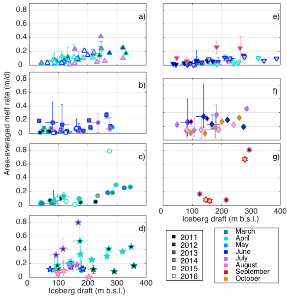
Figure 4: Area-averaged iceberg melt rate (meters per day) plotted against median draft (meters below sea level) for icebergs sampled near the terminus of (a) Kong Oscar Glacier, (b) Alison Glacier, (c) Upernavik Glacier, (d) Jakobshavn Isbræ, (e) Zachariae Isstrøm, (f) Helheim Glacier, and (g) Koge Bugt Glacier. For each observation period, icebergs were organized into 50 m-deep draft bins and the median melt rate and draft were computed. The symbols mark the median values and the error bars mark the range of estimates for each draft bin. The face colors and edge colors of the symbols indicate the year and month of the observations, respectively (see legends).
