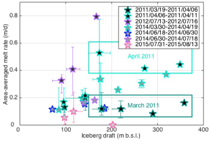
5 Figure 5: Area-averaged submarine melt rates plotted against median draft for icebergs calved from Jakobshavn Isbræ, west Greenland, into Ilulissat Isfjord. As in Figure 4, the symbols mark the median values and the error bars mark the range of estimates for each draft bin. The face colors and edge colors of the symbols indicate the year and month of the observations, respectively, as described in the legend. Deep melt rate estimates for the time period of rapid, significant change are circled for emphasis.
