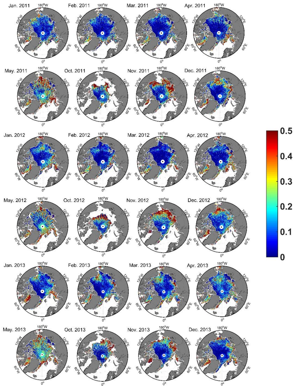
Figure 6: Monthly lead fraction maps based on waveform mixture algorithm from January to May, October to December between 2011 and 2013. The range of the colour bar was set from 0 to 0.5 to emphasize lower values.
