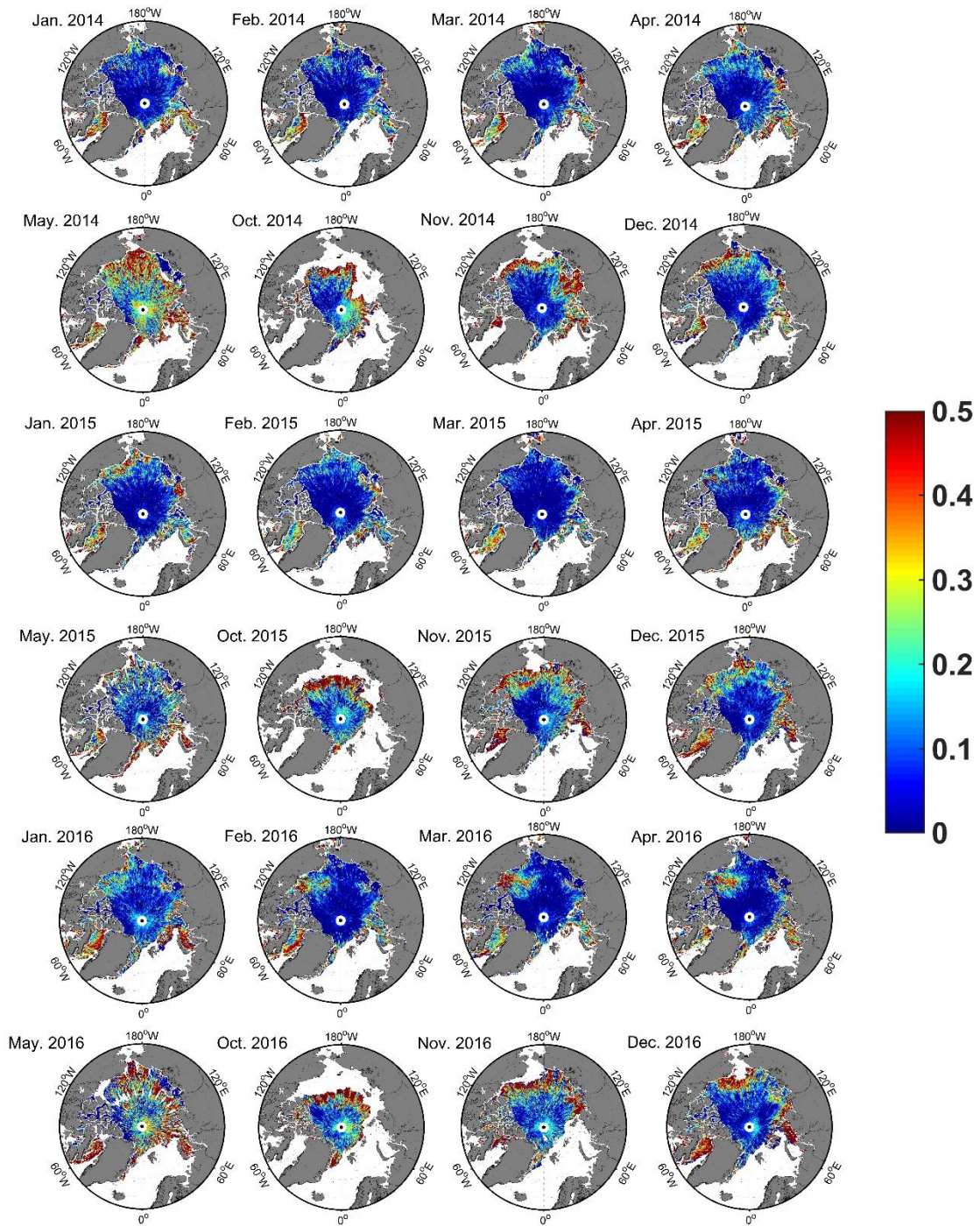
Figure 7: Monthly lead fraction maps based on waveform mixture algorithm from January to May, October to December between 2014 and 2016. The range of the colour bar was set from 0 to 0.5 to emphasize lower values.
