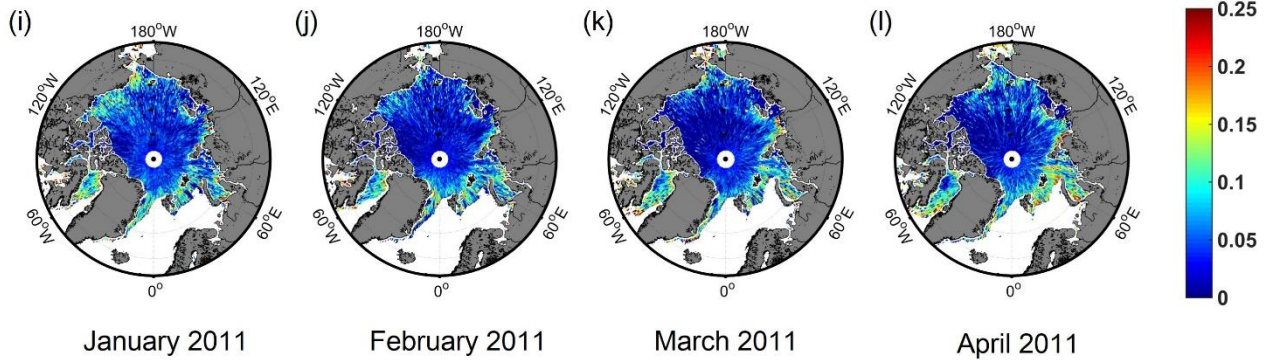
Figure 9: (a-d) the number of lead observations, (e-h) the number of ice observations, (i-l) the standard deviation of the results based on the sensitivity analysis of lead fraction from January to April 2011.
