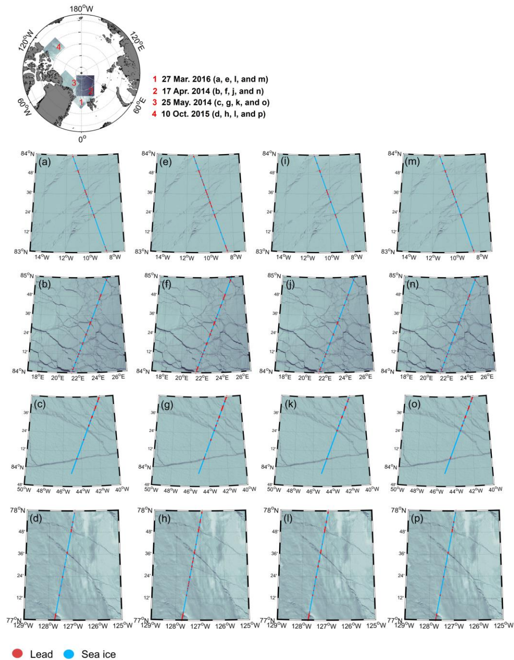
Response Fig. 3 Visual comparison of lead classifications: (a) – (d) lead classifications based on Rose (2013), (e) – (h) lead classifications based on Laxon et al. (2013), (i) – (l) lead classifications based on decision trees from Lee et al. (2016), and (m) – (p) lead classifications based on the proposed waveform mixture analysis. The MODIS data were collected on 27 March 2016 (a, e, i, and m), 17 April 2014 (b, f, j, and n), 25 May 2014 (c, g, k, and o), and 10 October 2015 (d, h, l, and p). An overview map of the location of cropped MODIS images is in top of the figure.
