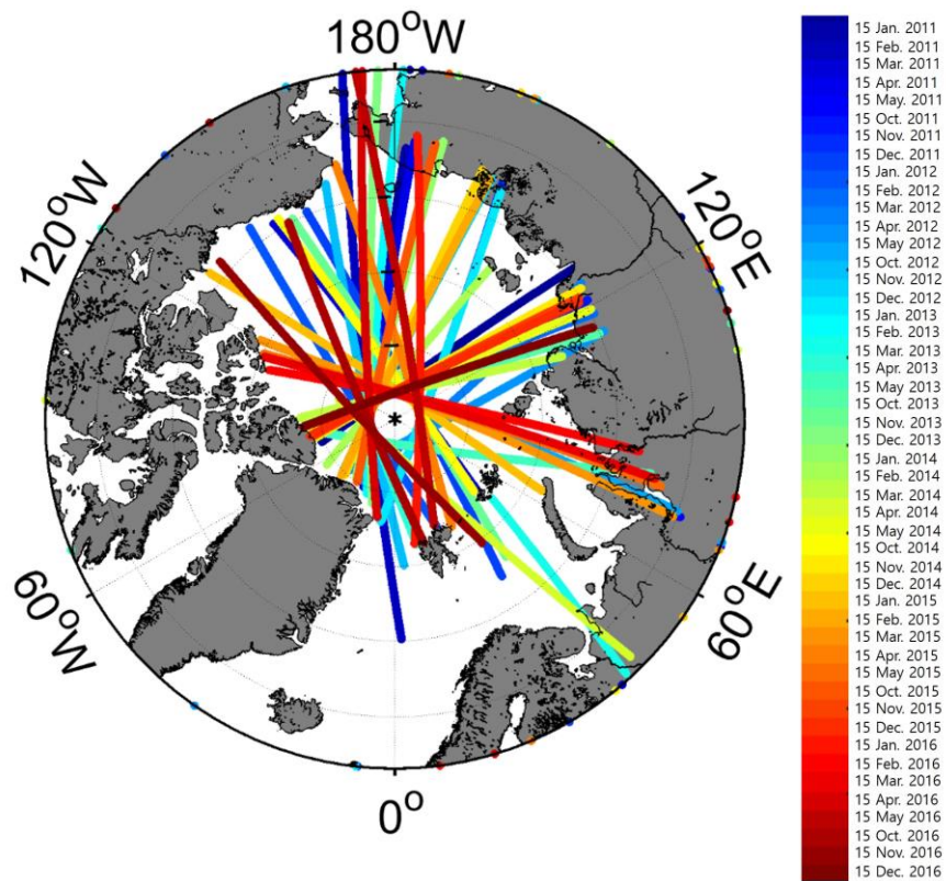
Response Fig. 1 The 48 CryoSat-2 orbit files from Jan. 2011 to Dec. 2016 used for extraction of endmember waveforms. The selected CryoSat-2 orbit files relatively cover the entire Arctic Ocean.
