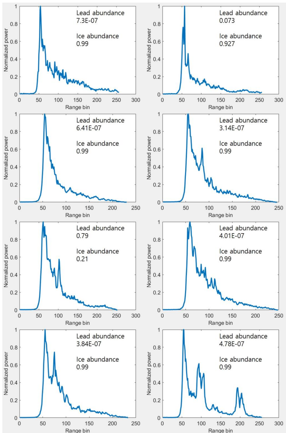
Fig. 2 The examples of multi-year sea ice waveforms from CryoSat-2 orbit files in 25 May 2014.
