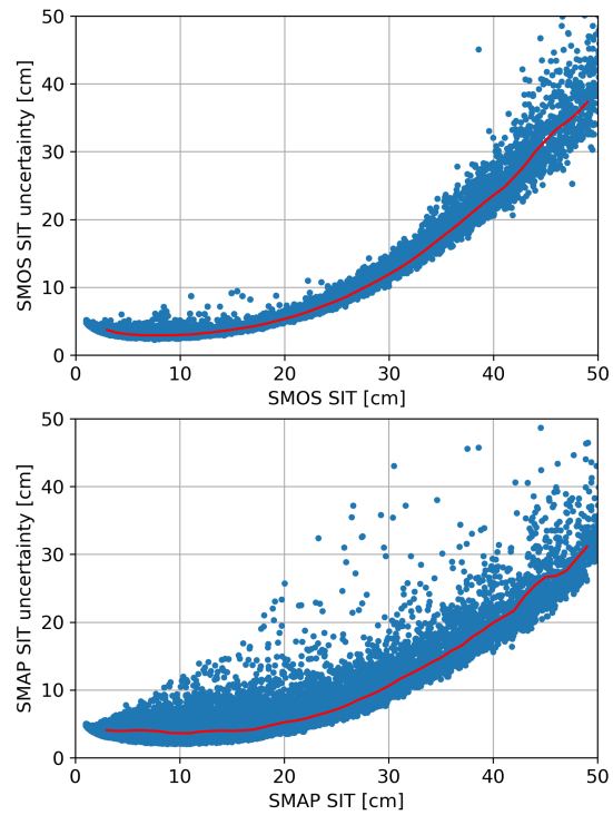
Figure 10. Scatter of SMOS (top) and SMAP (bottom) retrievals at 40^\circ incidence angle for 24 Oct. 2015 in the Arctic and their respective uncertainties. The red line shows the rolling average of the uncertainty.
