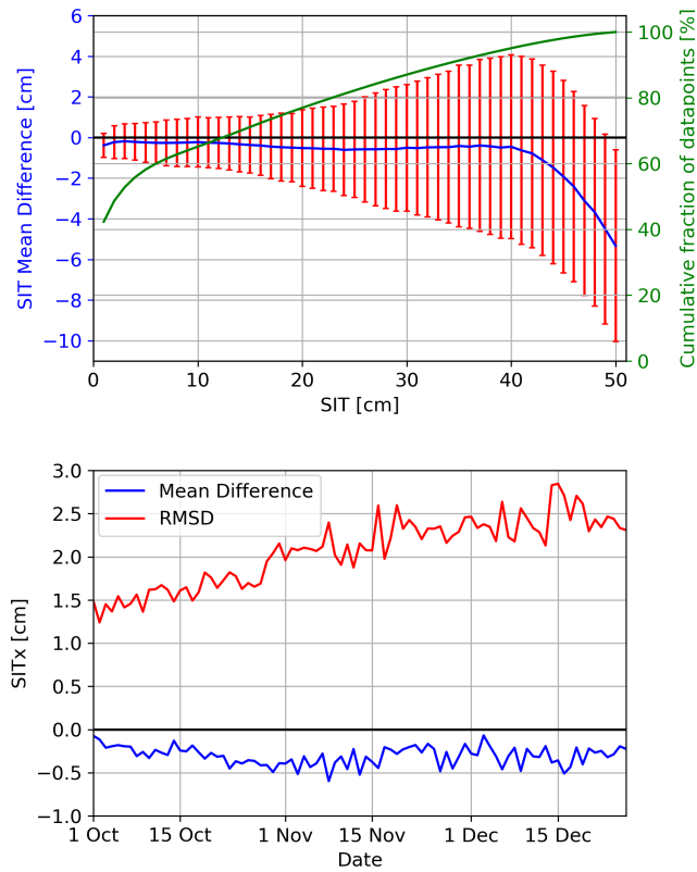
Figure 4. (Top) SIT bias-mean difference (blue) calculated by subtracting the SIT computed using 40-50° daily average from SIT using TBs fitted at 45° for the 1 Oct. to 26 Dec. 2010 period. Bias-Mean difference is computed relative to the daily average SIT in bins of 1 cm and its corresponding RMSD (red). Green curve represents the fraction from the total amount of data points for each thickness bin. Bottom figure shows the bias-mean difference (blue) and RMSD (red) for each day separately.
