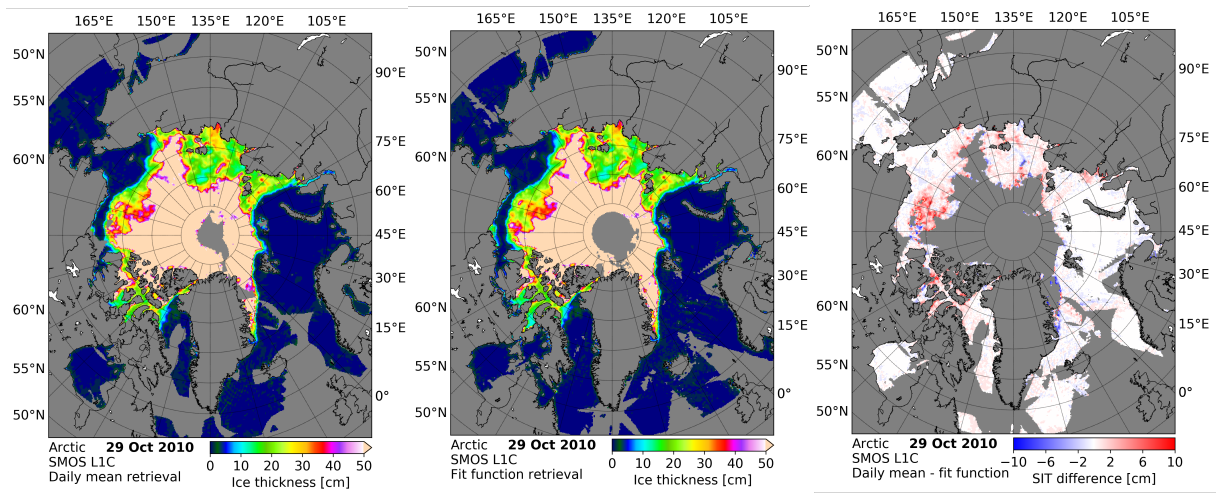
Figure 3. SMOS sea ice thickness retrieved on 29 October 2010 using 6.20 retrieval (left), retrieval using 45° incidence angle fitted brightness temperatures-TBs (central), and the difference between the two (right) with areas over 50 cm SIT not shown.
