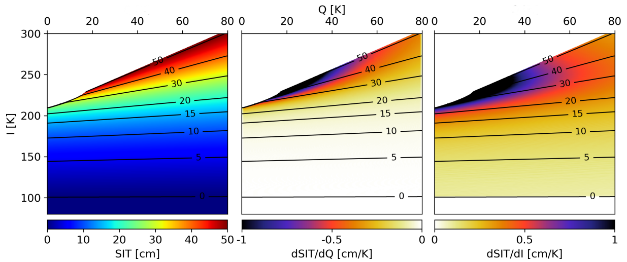
Figure 8. SIT (left) computed with the 40^\circ TB algorithm (Fig. 1 red curve) represented in the space of TB_n - Q and TB_v - I . Derivative of SIT as a function of TB_n - Q (center) and TB_v - I (right). Black line represents The black lines in all three figures represent the location isolines of equal TB_n and TB_v , with the area above SIT derived from the line ( TB_v higher than TB_n ) representing values found in observations left figure.
