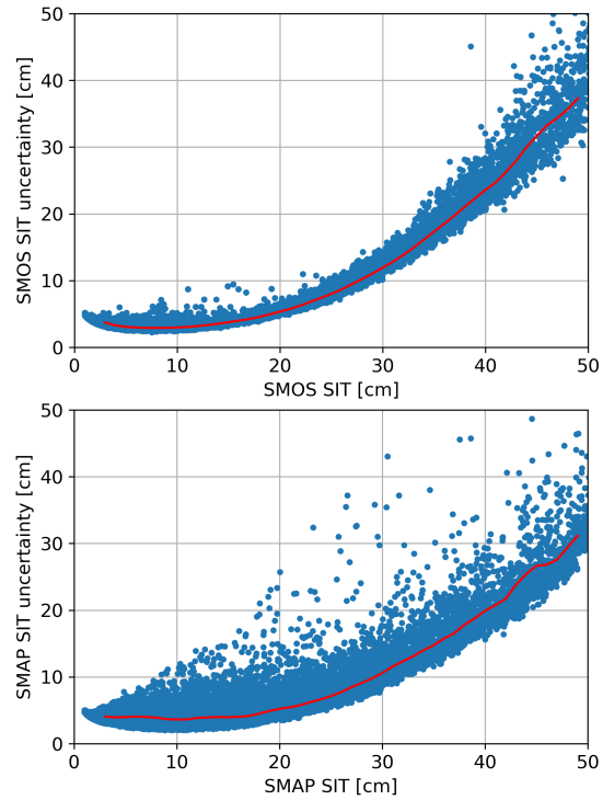
Figure 10. Scatter of SMOS (top) and SMAP (bottom) retrievals at 40° incidence angle for 24 Oct. 2015 in the Arctic and their respective uncertainties. Red line represent the rolling average of the uncertainty.
