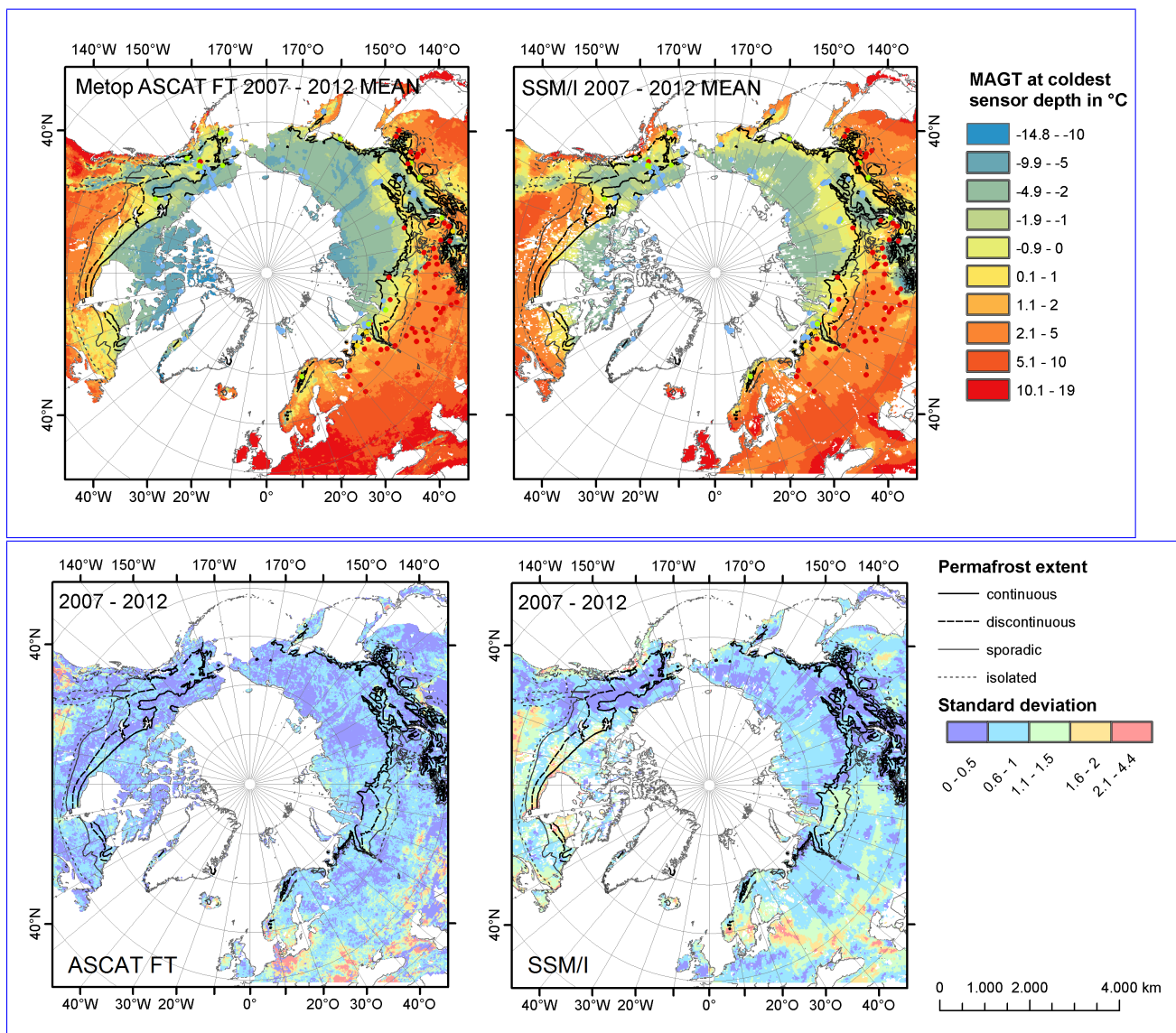
Figure 13. Comparison Maps of satellite data results based on modelled mean annual ground temperatures with temperature (top) and standard deviation of modelled MAGT c (bottom) for ASCAT excluding melt days (FT; left) and SSM/I (right) based on all analyzed years. Source for permafrost extent from classes: Brown et al. (1997). Covered area in % inside and outside permafrost regions. FT - days identified as frozen without melting snow are used, FM - days with melting snow are considered as frozen ground, LM - model results.
