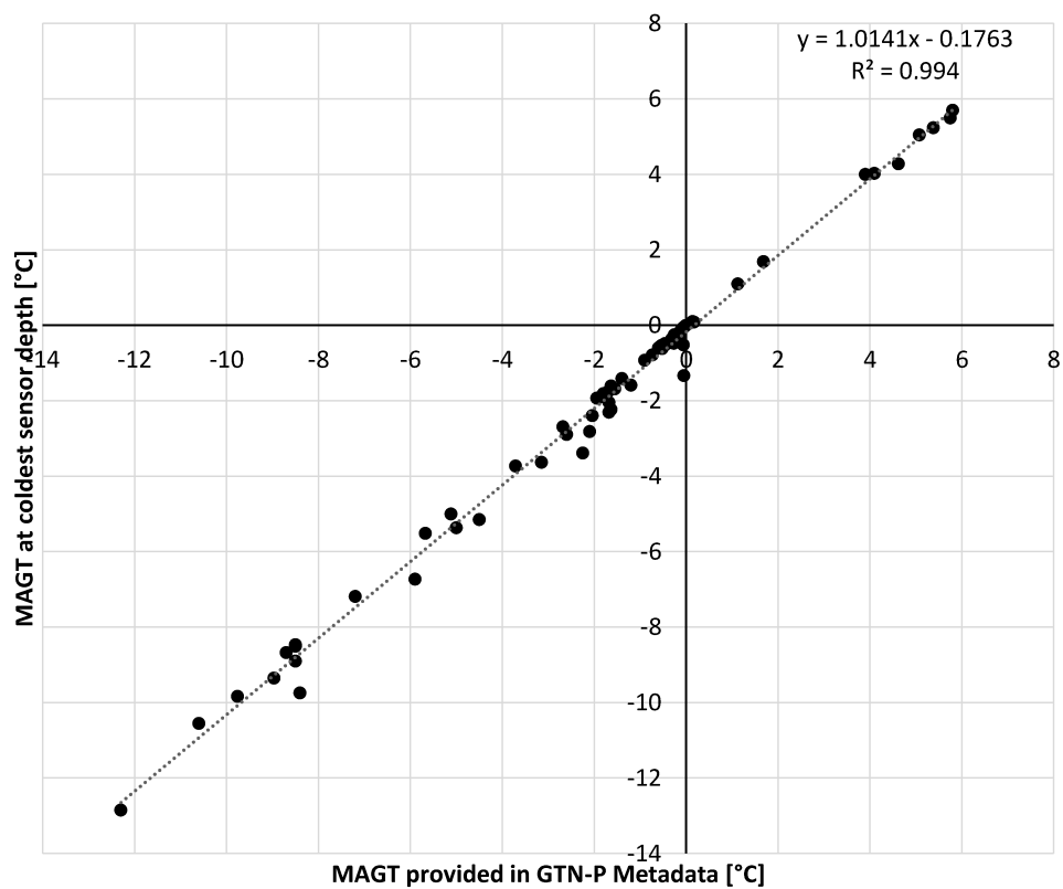
Figure 1. Mean Annual Ground Temperature (MAGT) derived from GTN-P -metadata ( at or close to zero annual amplitude ) versus derived MAGT c from coldest sensor (for year of MAGT specified in the meta data) based on GTN-P borehole records . Dotted line represents linear fit.
