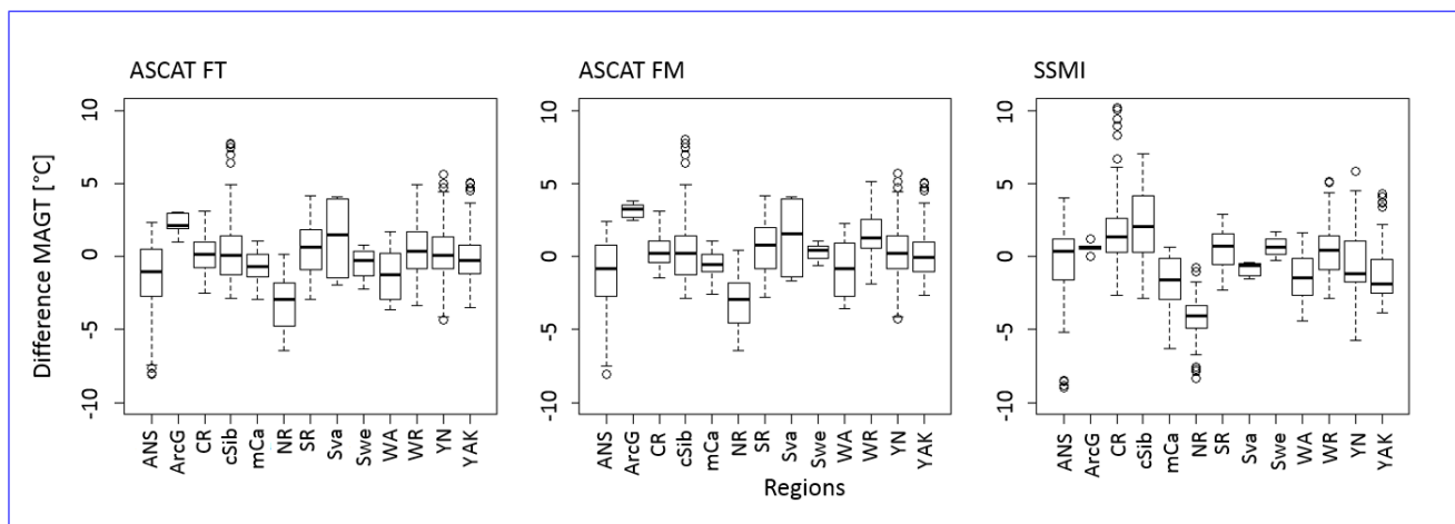
Figure 8. Difference between in situ MAGT c (coldest sensor) and modelled MAGT c by region (see Fig. A1 for abbreviations and map) for all years. Only stations which overlap with records from all datasets are considered. FT - days identified as frozen without melting snow are used, FM - days with melting snow are considered as frozen ground in ASCAT.
