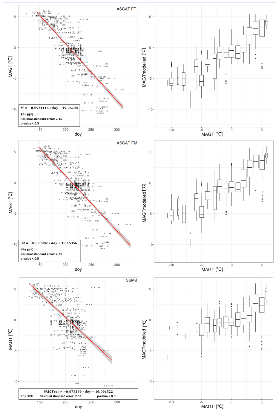
Figure 2. Left: Comparison of number of frozen days (doy - days of year) from satellite records and Mean Annual Ground Temperature for GTN-P boreholes (at depth of coldest sensor, years 2010-2012). Red line represents linear fit. Right: Box plots of modeled versus Mean Annual Ground Temperature from GTN-P boreholes (at depth of coldest sensor, years 2007/8 and 2008/9) Top: ASCAT excluding snow melt days, middle: ASCAT with snow melt days, bottom: SSM/I.
