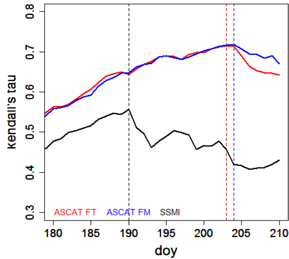
Figure 11. Curves of correlation coefficient (Kendall's \tau ) between 180 and 210 day of year (day) frozen from satellite products and positive or negative MAGT c at depth of coldest sensor from borehole data. FT - days identified as frozen without melting snow are used, FM - days with melting snow are considered as frozen ground with Metop ASCAT.
