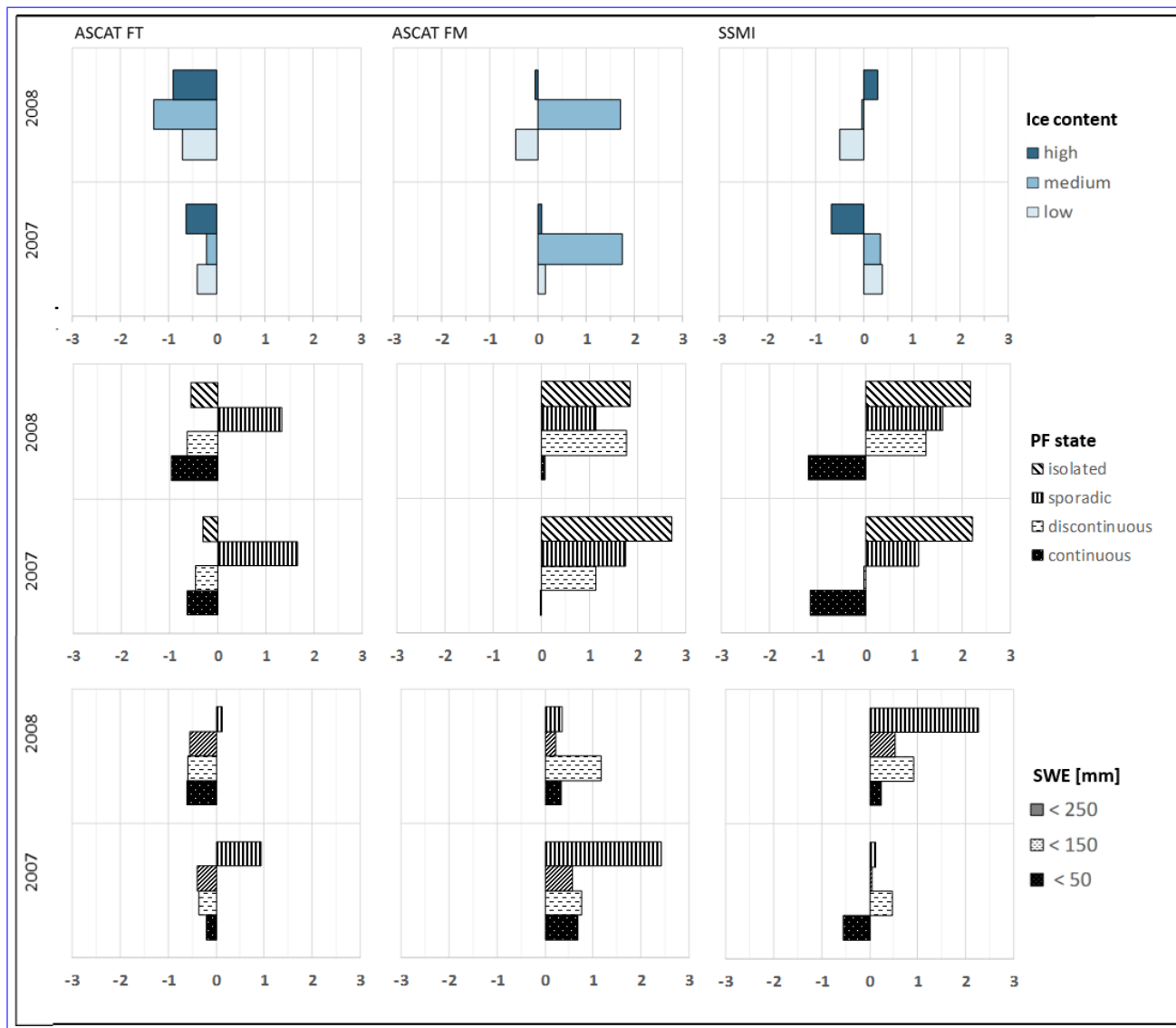
Figure 9. Difference between in % inside-situ MAGT c (coldest sensor) and outside-modelled MAGT c (coldest sensor) by permafrost regions is provided, zone and ice content (source: Brown et al. (1997)), and snow water equivalent (SWE, source: GlobSnow) categories in 2007/8 and 2008/9. FT - days identified as frozen without melting snow are used, FM - days with melting snow are considered as frozen ground with Metop-in ASCAT.
