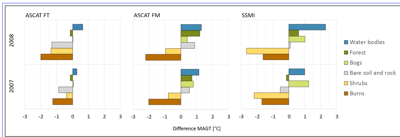
Figure 14. Difference between in situ MAGT_c (coldest sensor) and modelled MAGT_c by land cover type (source: GLC2000 (2003)) in 2007/8 and 2008/9. FT - days identified as frozen without melting snow are used, FM - days with melting snow are considered as frozen ground in ASCAT.
