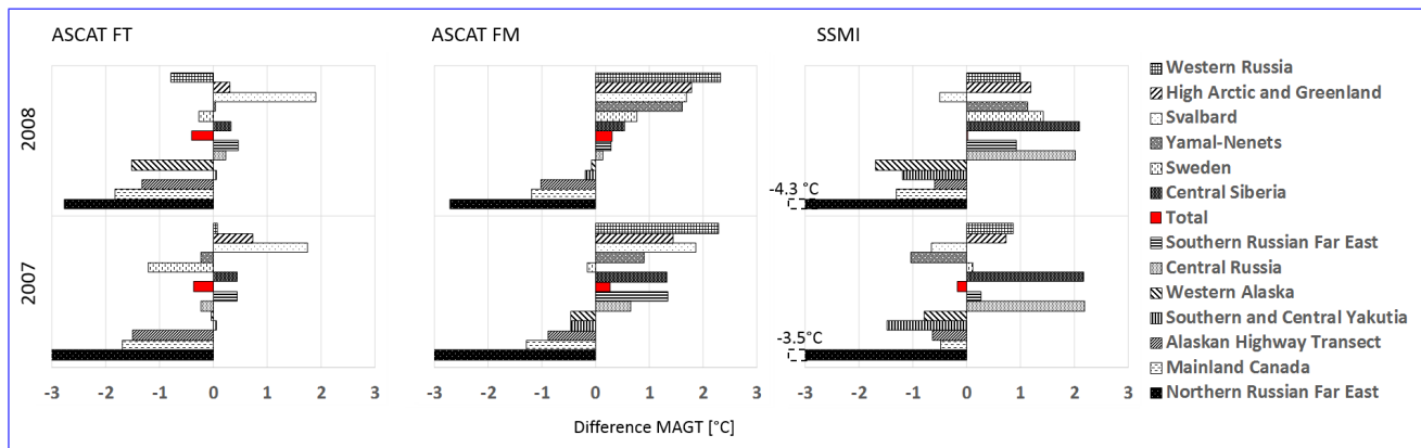
Figure 4. Difference between in situ MAGT_c (coldest sensor) and modelled MAGT_c by region (see Fig. A1) in 2007/8 and 2008/9. FT - days identified as frozen without melting snow are used, FM - days with melting snow are considered as frozen ground in ASCAT.
