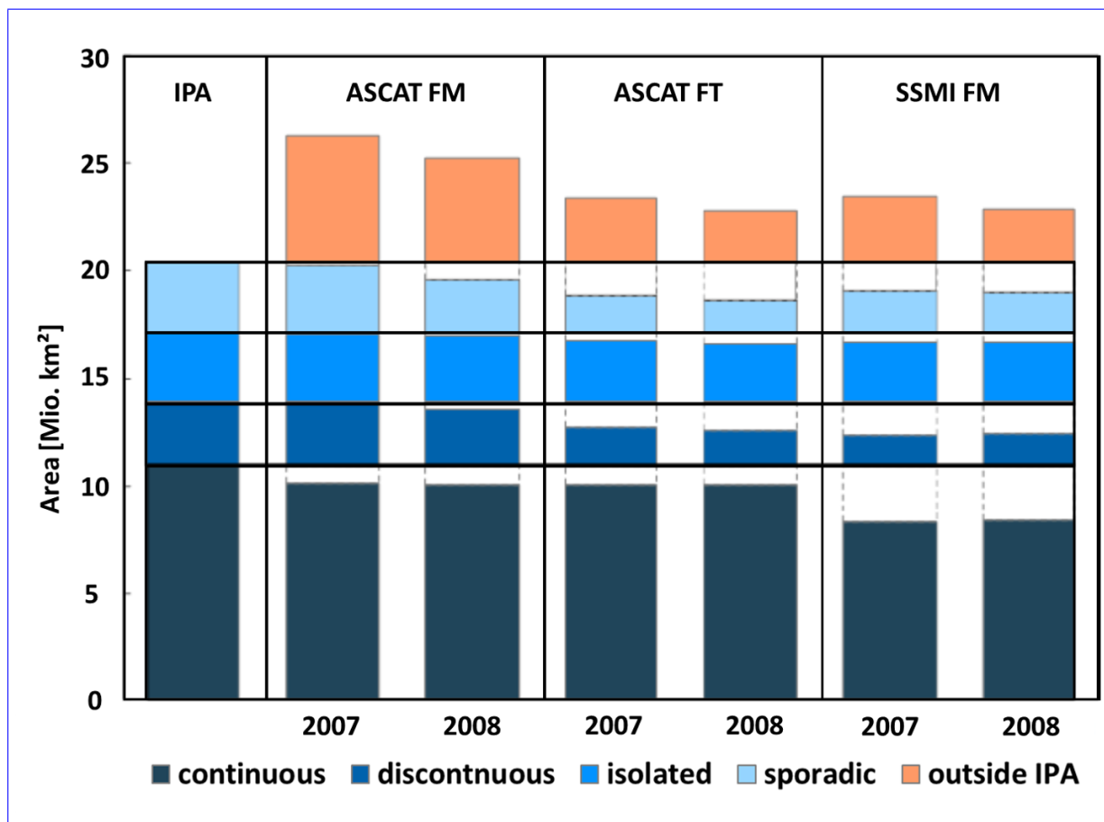
Figure 12. Permafrost extent comparison of satellite data results based on modelled ground temperatures (LM - Linear Model) with permafrost classes from Brown et al. (1997). Covered area in km 2 within each class and outside. FT - days identified as frozen with ASCAT, FM - days with melting snow are considered as frozen ground with ASCAT.
