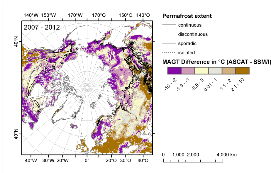
Figure 3. Comparison of MAGT_c (coldest sensor) in °C of all years between Metop ASCAT (FT) and SSM/I for 2007-2012. Source of permafrost extent classes: Brown et al. (1997).
