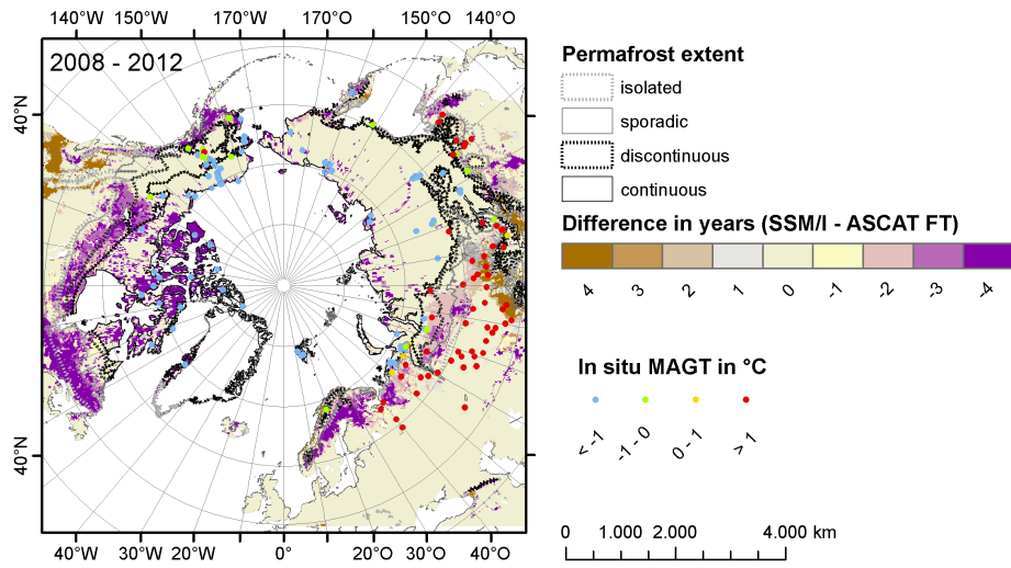
Fig. 2. Permafrost extent comparison of satellite data results from Metop ASCAT and SSM/I for 2008-2012 based on the original 180 day threshold method applied to all years
