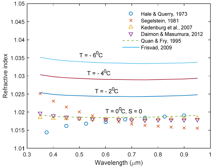
5 Figure 1. Spectra of the relative refractive index 'water-to-ice': distilled water (symbols), fresh water at 0°C (dashes), and brine with equilibrium salinity at different temperatures (solids).
