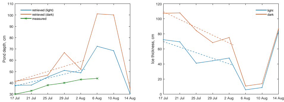
Figure 12. Retrieved pond depth (left) and ice thickness (right) for the two parts of the dual pond shown in Fig. 12. The measured pond depth is shown with crosses. The dashed lines show the linear regression for the first 5 dates.
