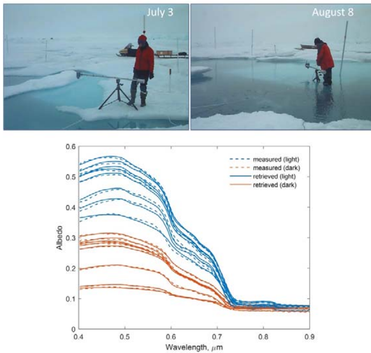
Figure 11. SHEBA-1998 dual pond: photos and spectra, measured (dashed) at the light (blue) and dark (red) parts and simulated (solid). The photographs are taken at the early and late melt season (on July 3 and August 8, respectively).
