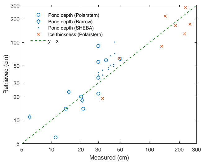
Figure 13. Ice thickness and pond depth, measured at different stations and retrieved. For ice thickness R^2 = 0.56 ( N=8 ) and for pond depth R^2 = 0.62 ( N=26 ).
