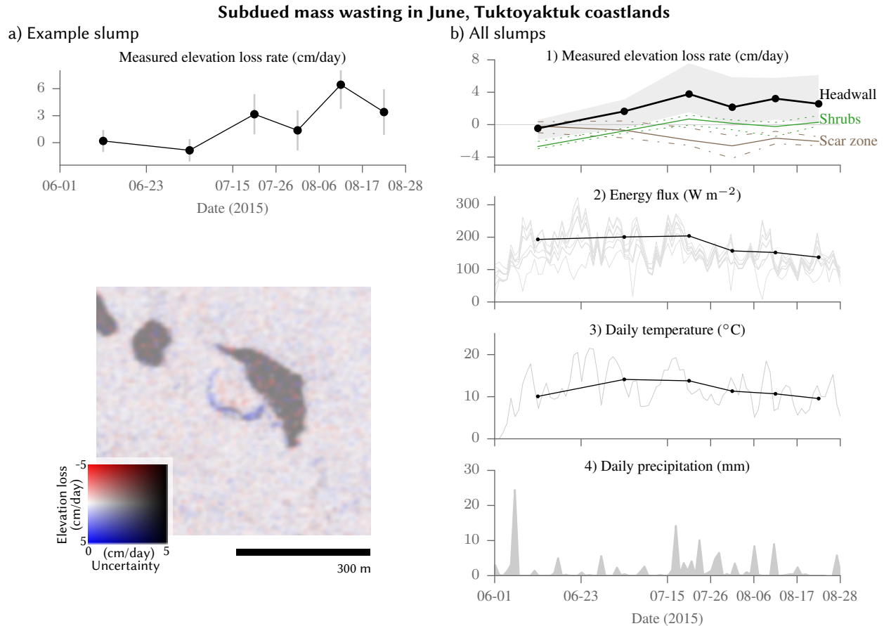
Figure 4. Observed time series of elevation losses in the Tuktoyaktuk coastlands. a) Sub-seasonal elevation loss rates r at thaw slump 152 (see Fig. 3) are lower in June and early July than later in summer. The rates r are plotted halfway between the differenced successive TanDEM-X acquisitions (shown by ticks). The elevation losses occur at the arcuate headwall, as shown below (stacked losses r_s between mid-July and August). b) 1) Spatially aggregated sub-seasonal elevation loss rate r at thaw slumps covered by the ascending orbit ( N = 71 ; solid black line: median, grey area: interquartile range), along with observed rates over all slump scar zones with detected changes ( N = 25 ) and over patches with dense shrub cover ( N = 10 ). The observed elevation loss rate is plotted halfway between the earlier and the later acquisition (indicated by ticks). 2) Available energy for different headwall orientations (grey) and temporal averages for a horizontal surface (black). 3) Temperature at Inuvik (daily averages in grey; averages between subsequent acquisitions in black). 4) Daily precipitation measured in Inuvik. .
